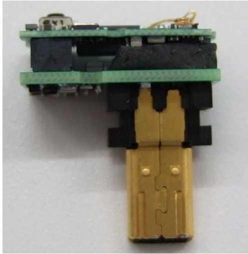
RF Board+Connector Board (Side A)
