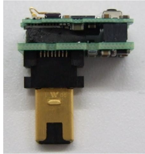
RF Board+Connector Board (Side C)
