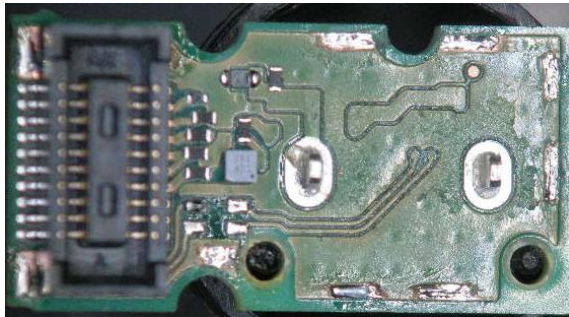
Connector Board(Top)
