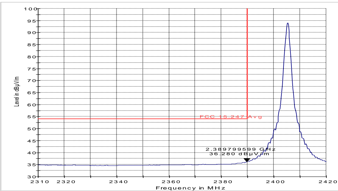
FCC 15.247 LBE Avg 3m
