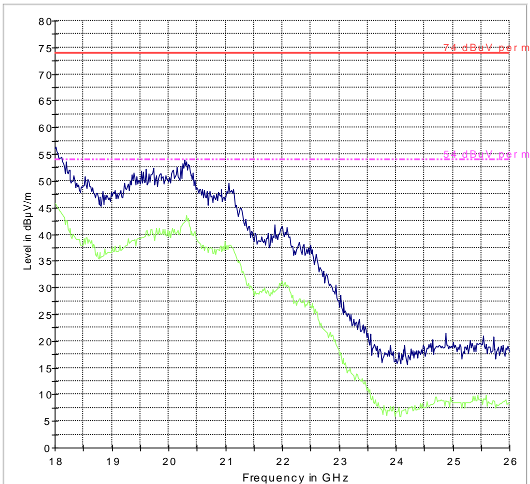
FCC 15 18-26GHz
