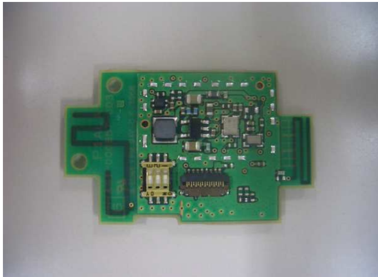
P1ALA PCBA—A Side
