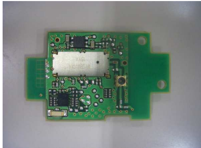
P1ALA PCBA—B Side
