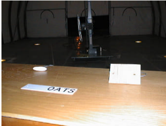
Figure 6.15 - Radiated Emissions, Open Area Test Site (NX1700)
