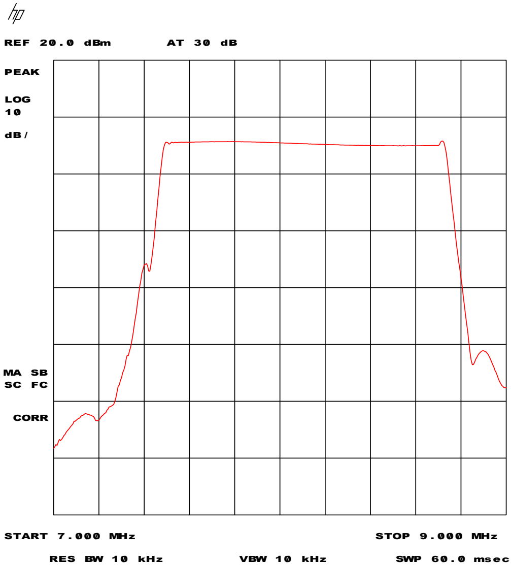
Figure 4 Plot of the 8 MHz sweeping signal
