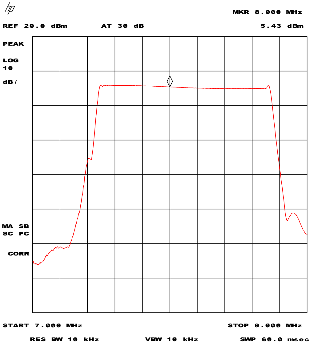
Figure 6 Plot of the 8 MHz sweeping signal
