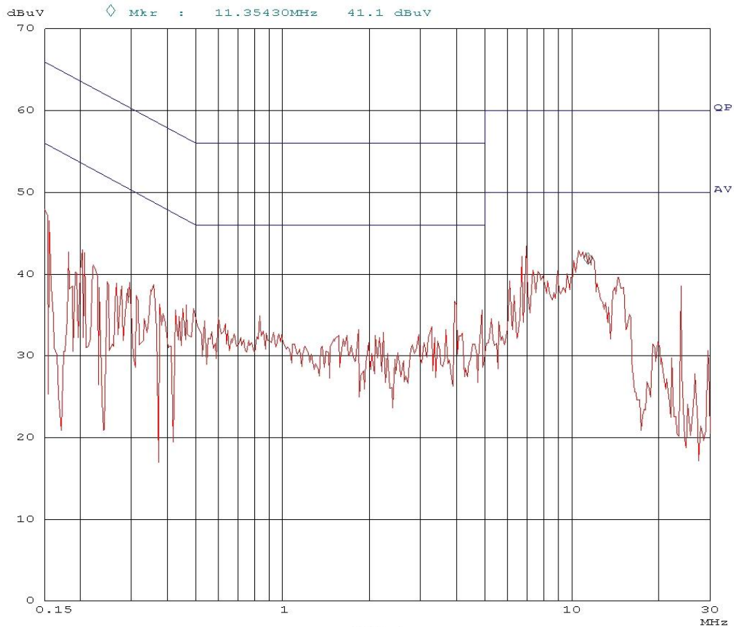
Conducted emissions on L1
