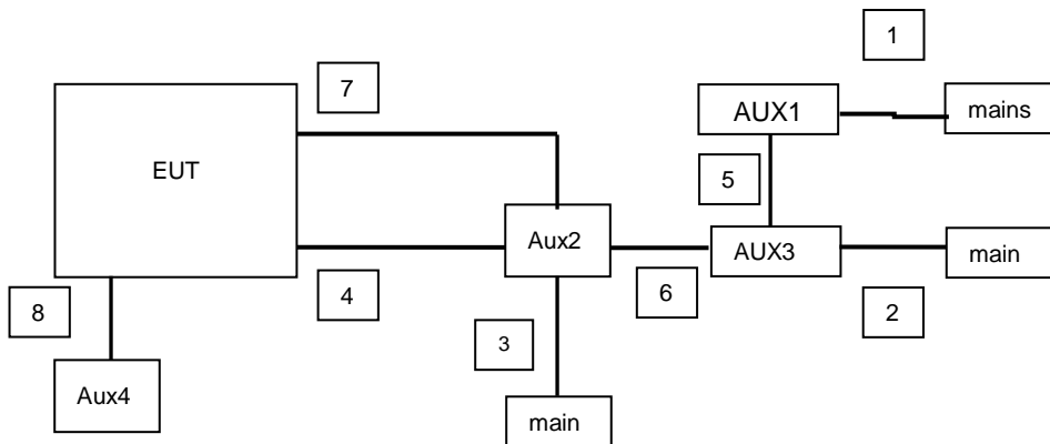
Figure 1. Basic set-up
