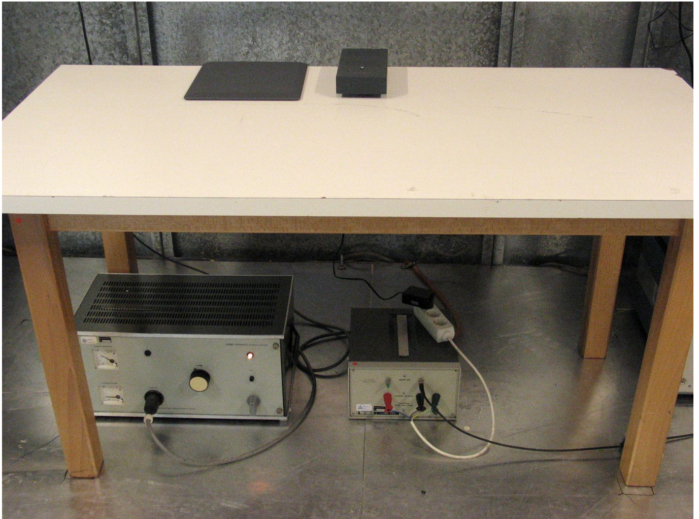
Conducted emission setup, front view
