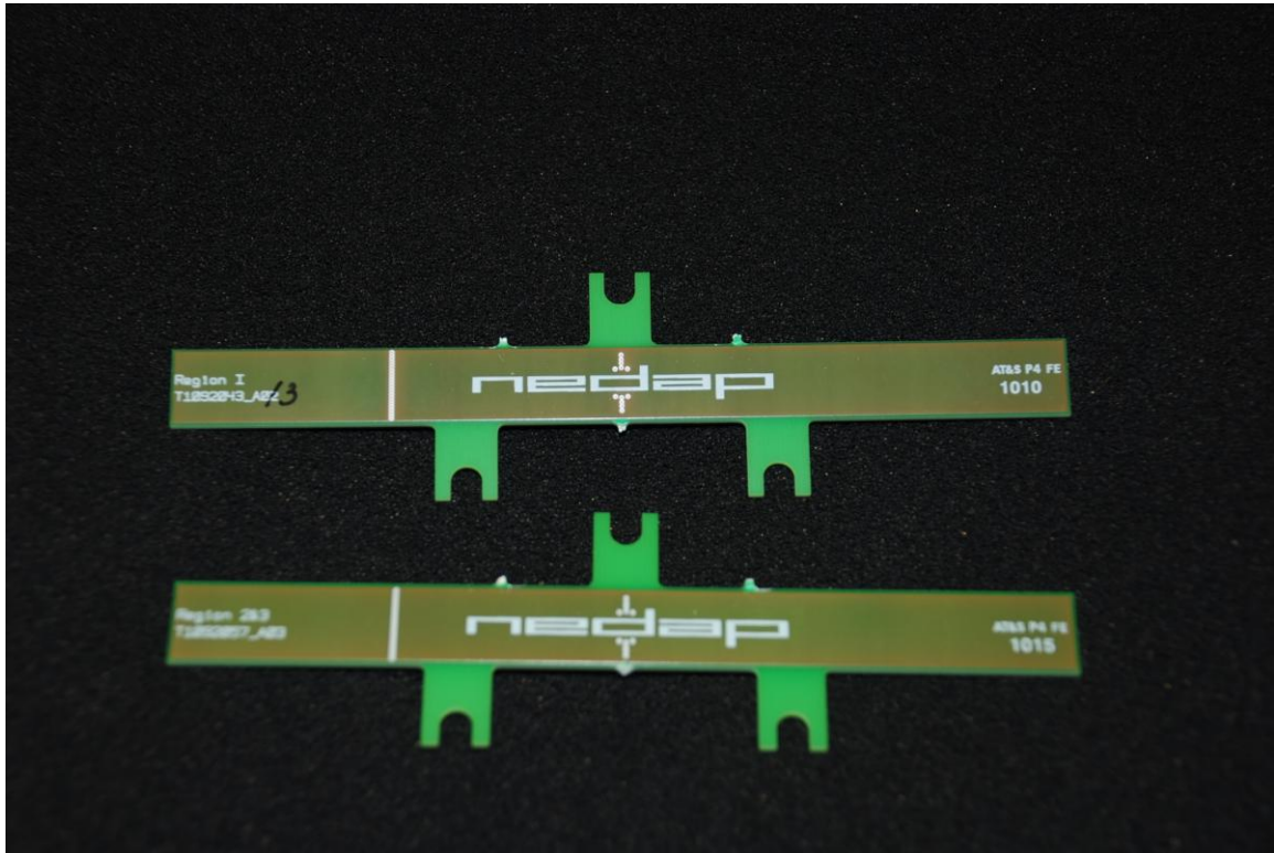
Photograph 7: UHF dipole antenna, top view
