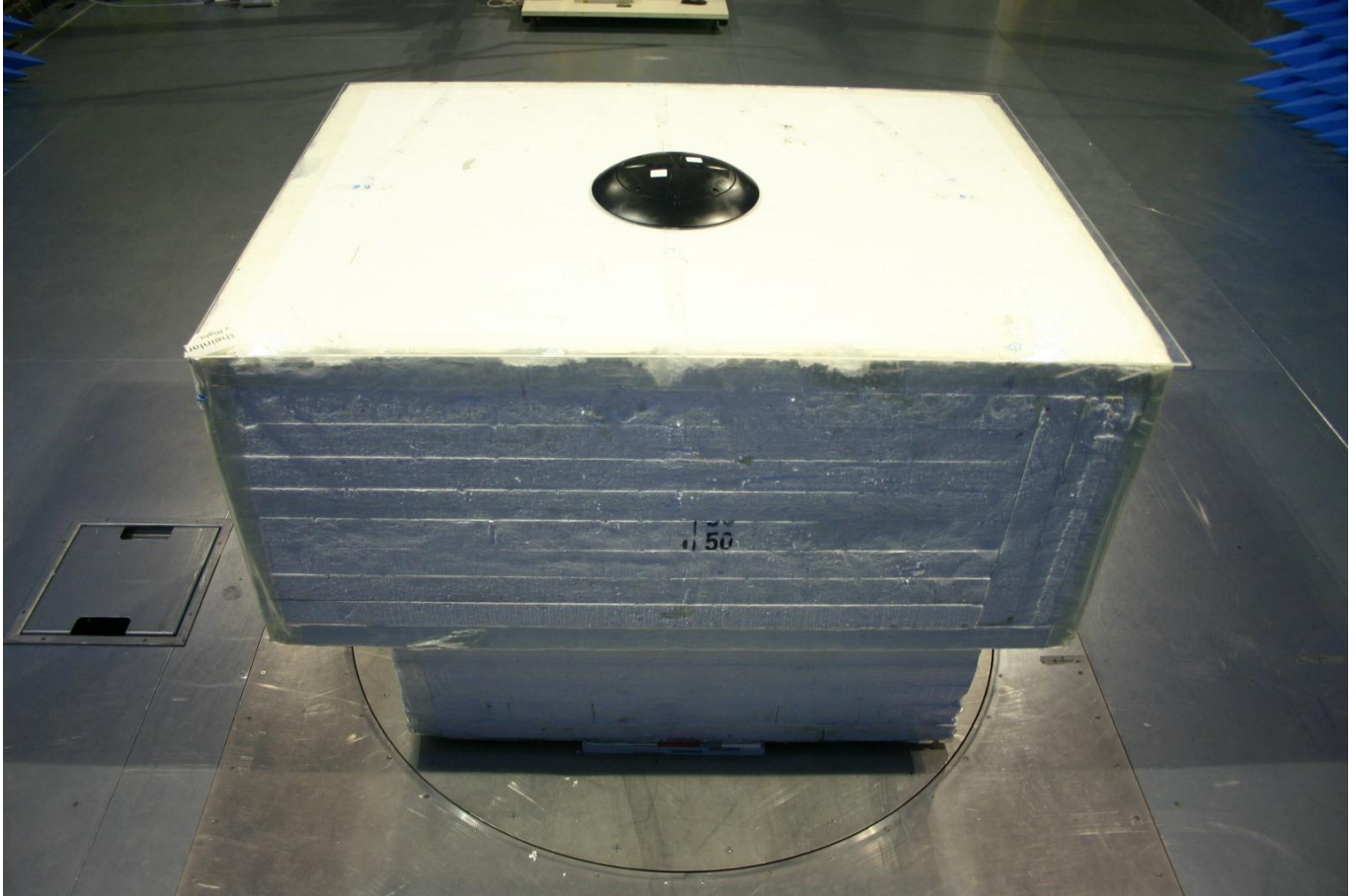
Rear view of the EUT setup
