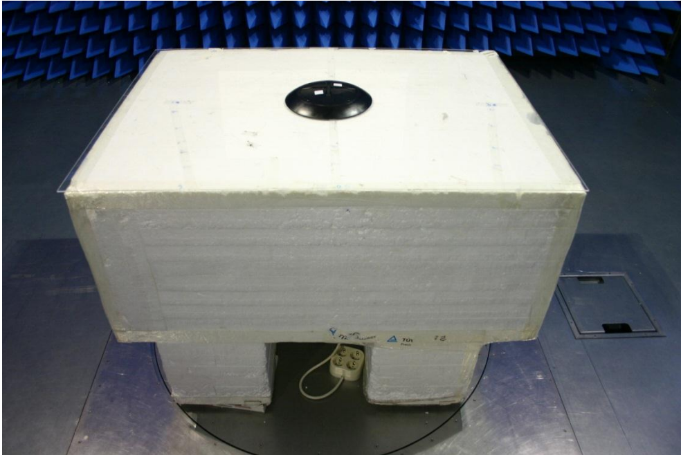
Front view of the EUT setup, EUT horizontal
