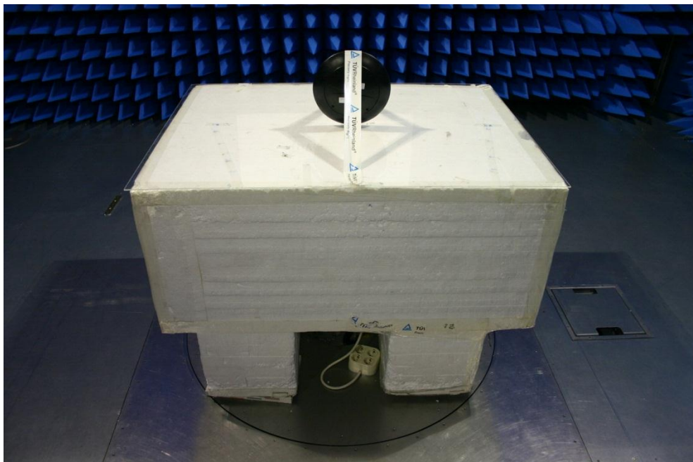
Front view of the EUT setup, EUT vertical
