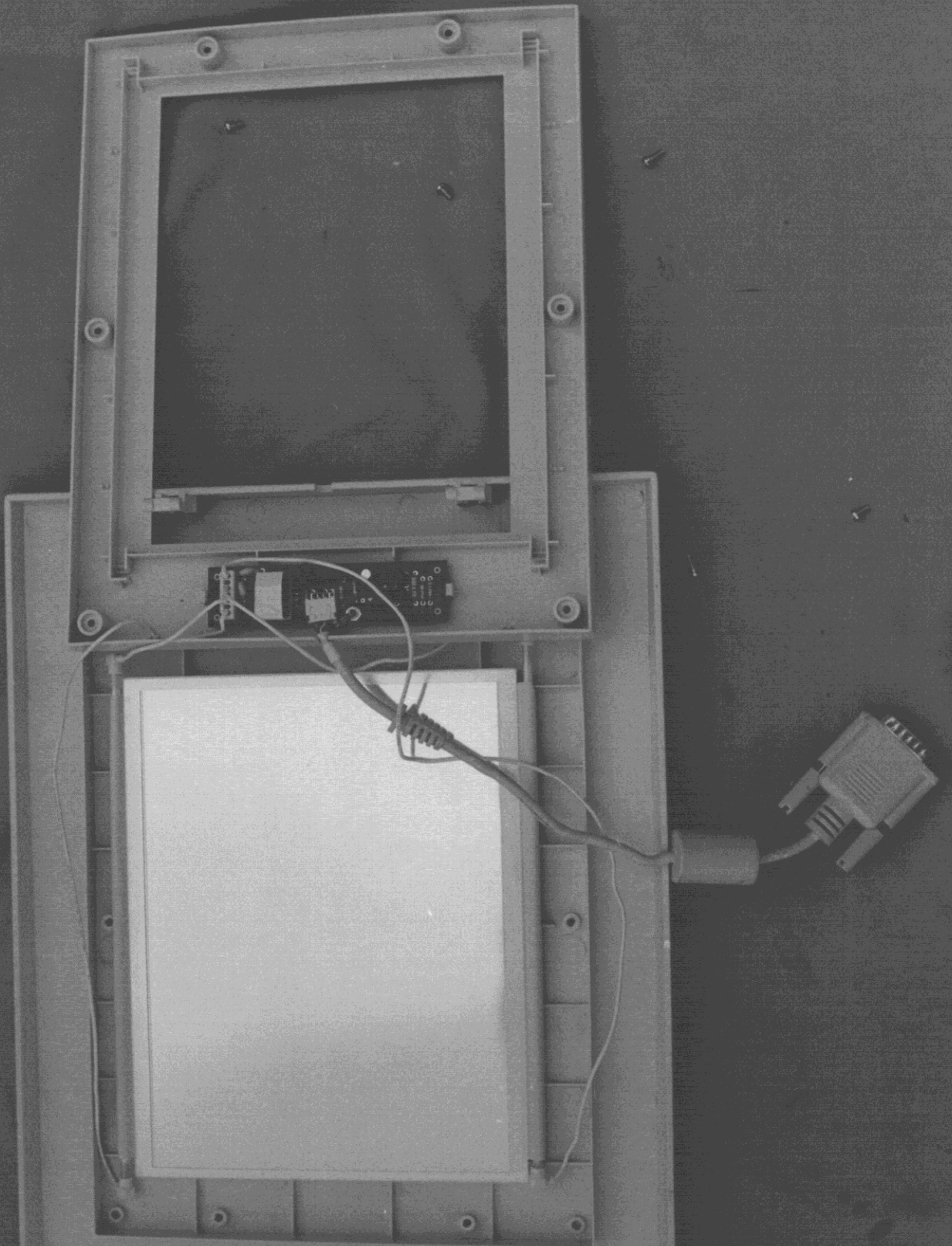
Figure 20 Cover Removed, Internal View of Light Plate
