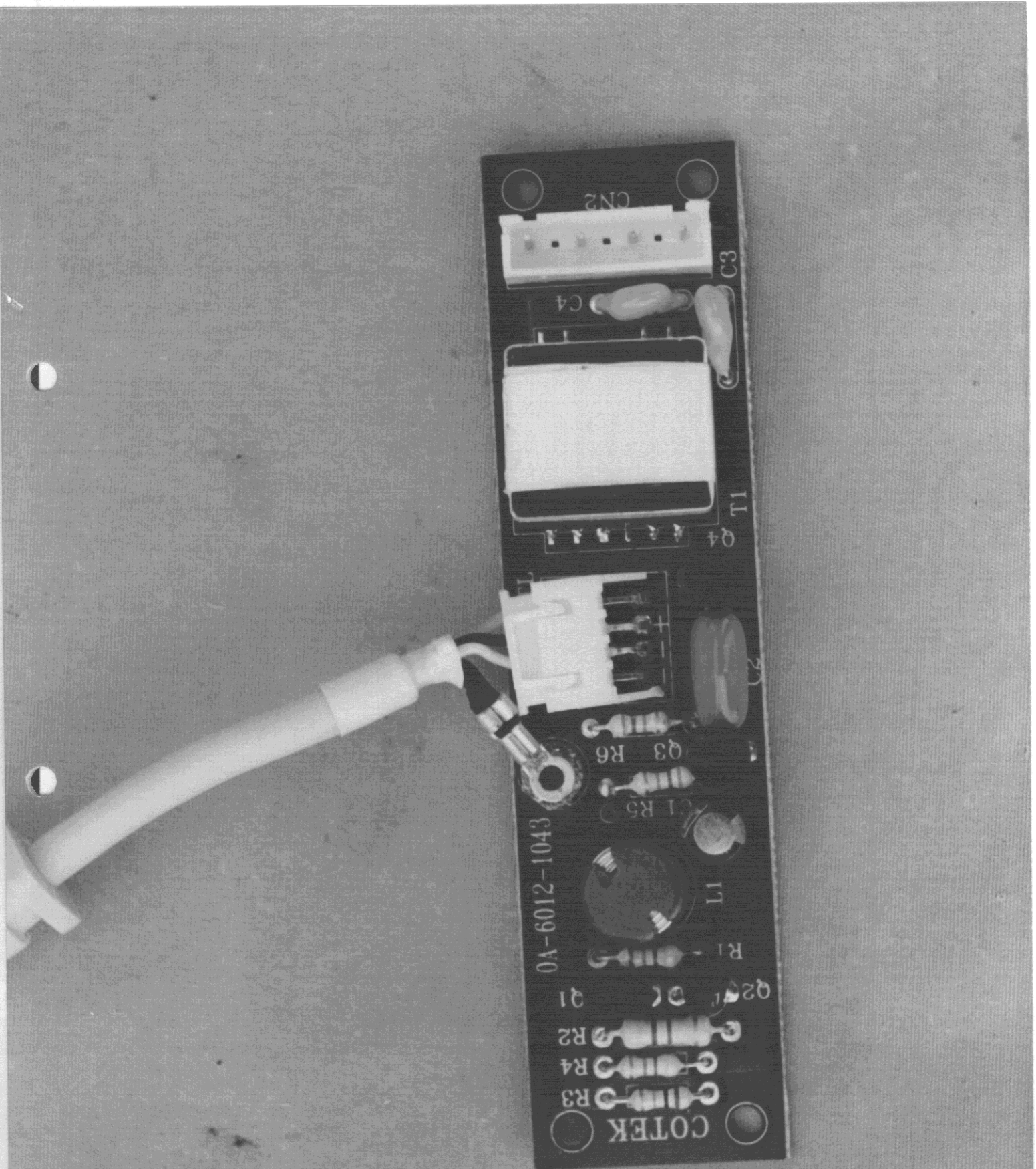
Figure 22 Control Board of Light Plate
