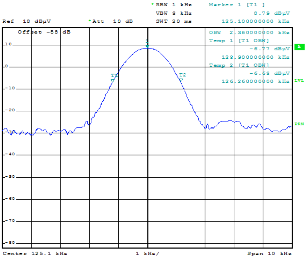
Plot 2b: 99% bandwidth of the 125.1 kHz Metal detection system is 2.36 kHz as measured on a spectrum analyzer
