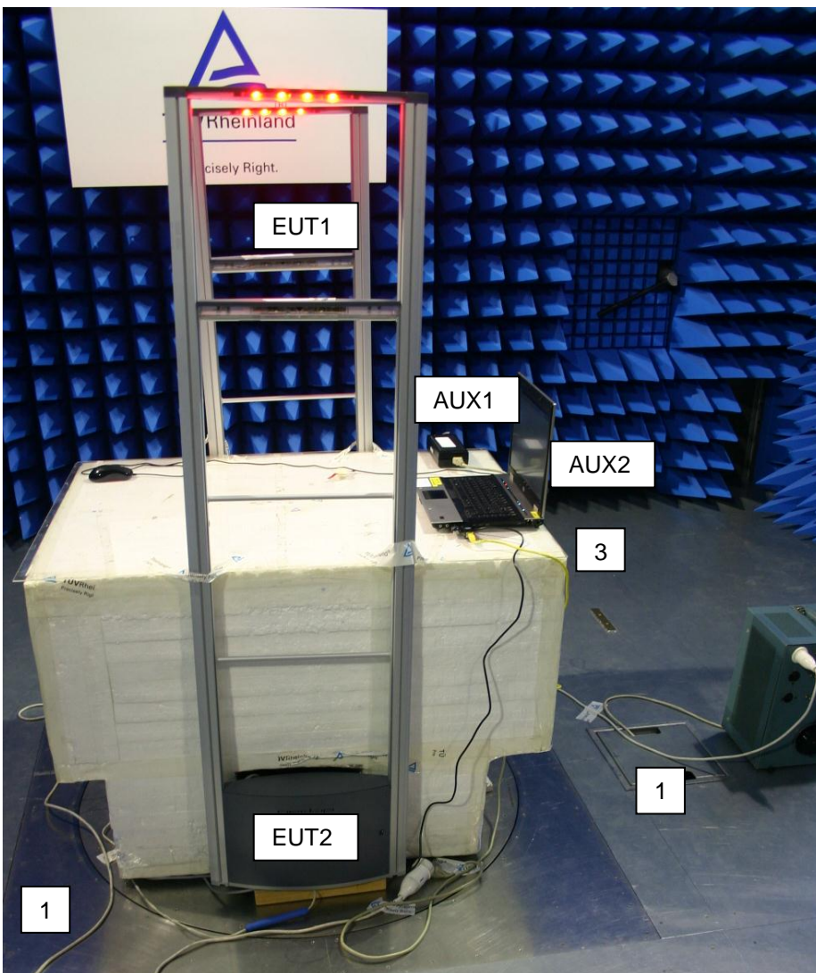
Photographs of the EUT in the testsetup (schematic overview is given on the next page). Tested with and without AUX2. AUX2 is only required for making testsettings.
