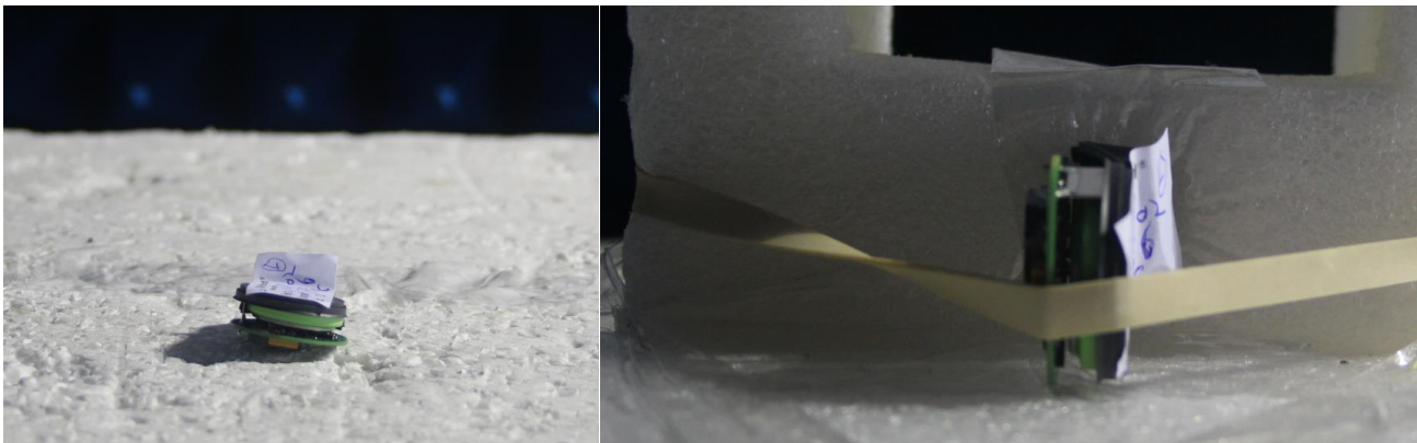
EUT in the horizontal position (left) and Z-position (right)
