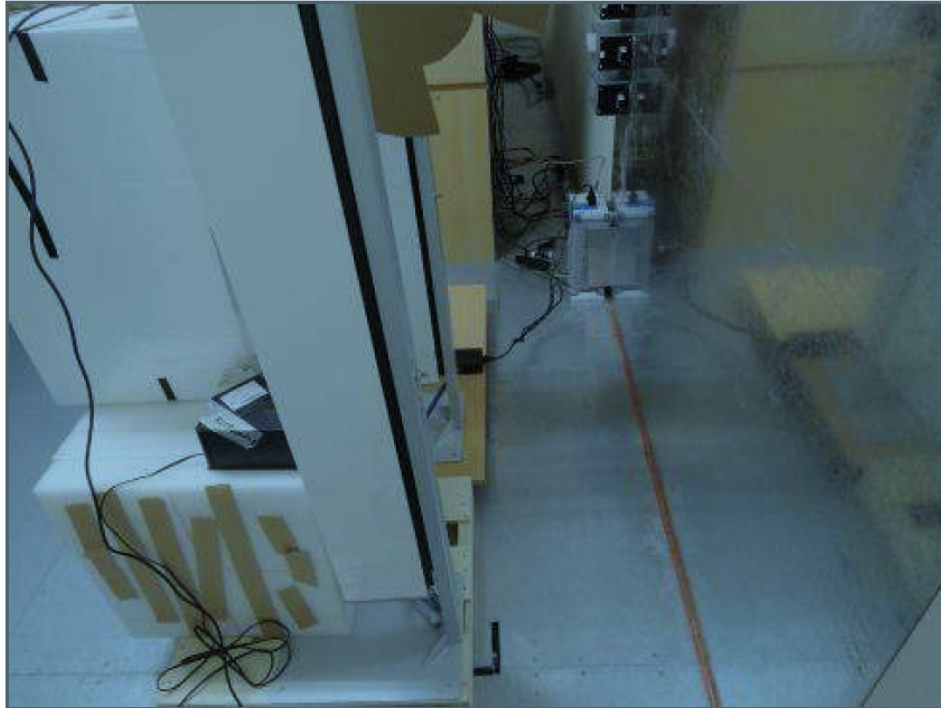
Photograph 4: Set-up for Mains Conducted testing Back
