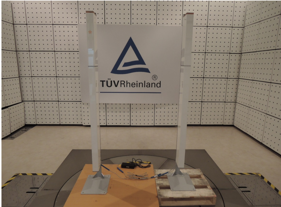
Photograph 1: Set-up for Spurious Emissions TX (Front View)
