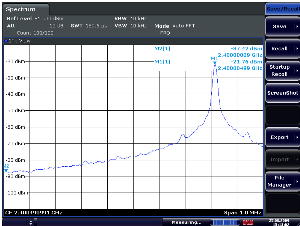
Plot of the lower band edge
