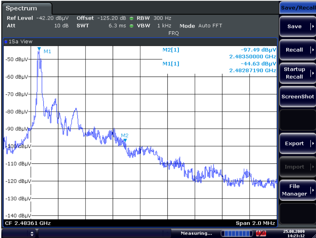
Plot of the higher band edge
