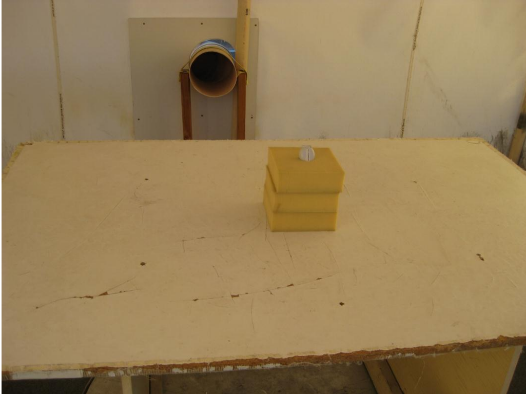
Radiated Emissions #1
