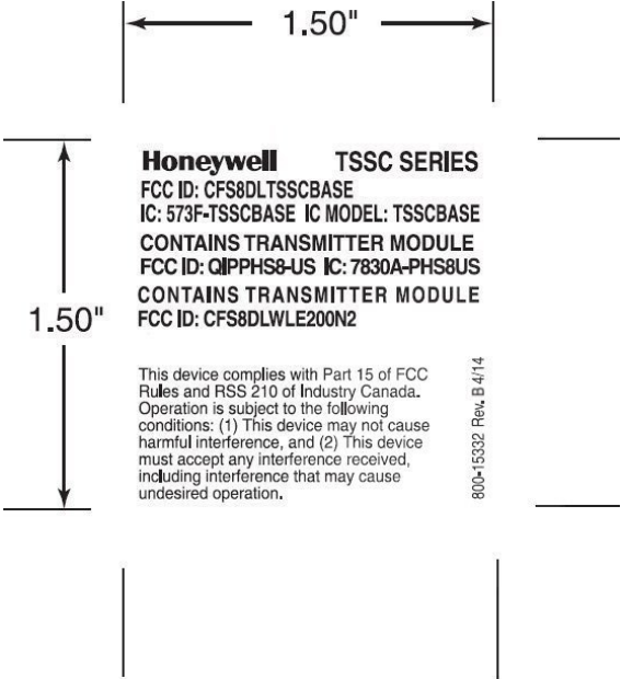
CASE BACK
