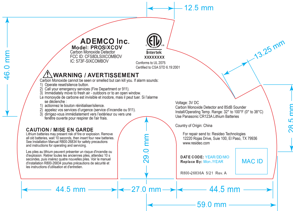
R800-26836A 5/21 Rev A PROSIXCOV_Carbon Monoxide Detector
