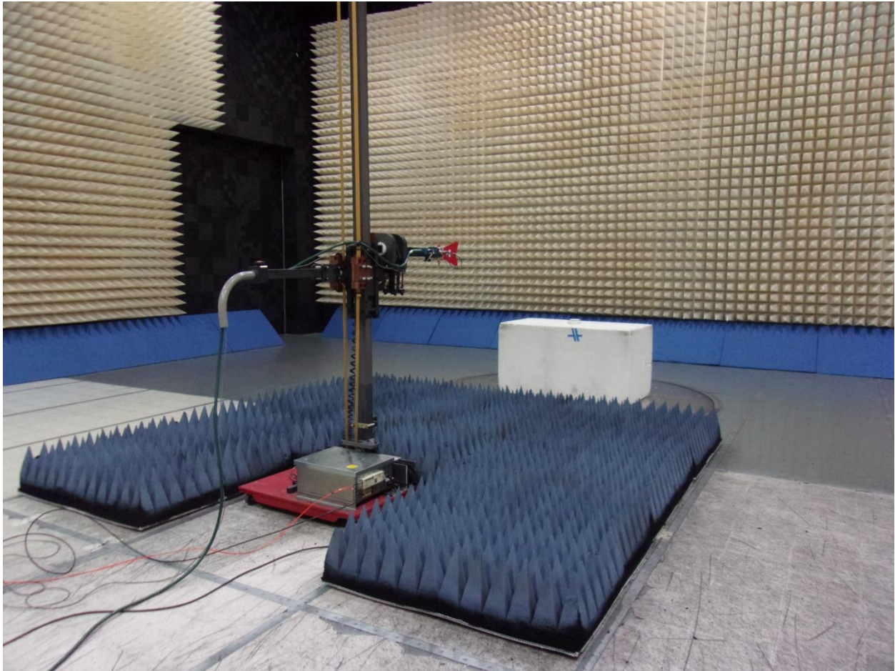
Radiated Emissions: 1GHz-18GHz (Transmitter Idle)
