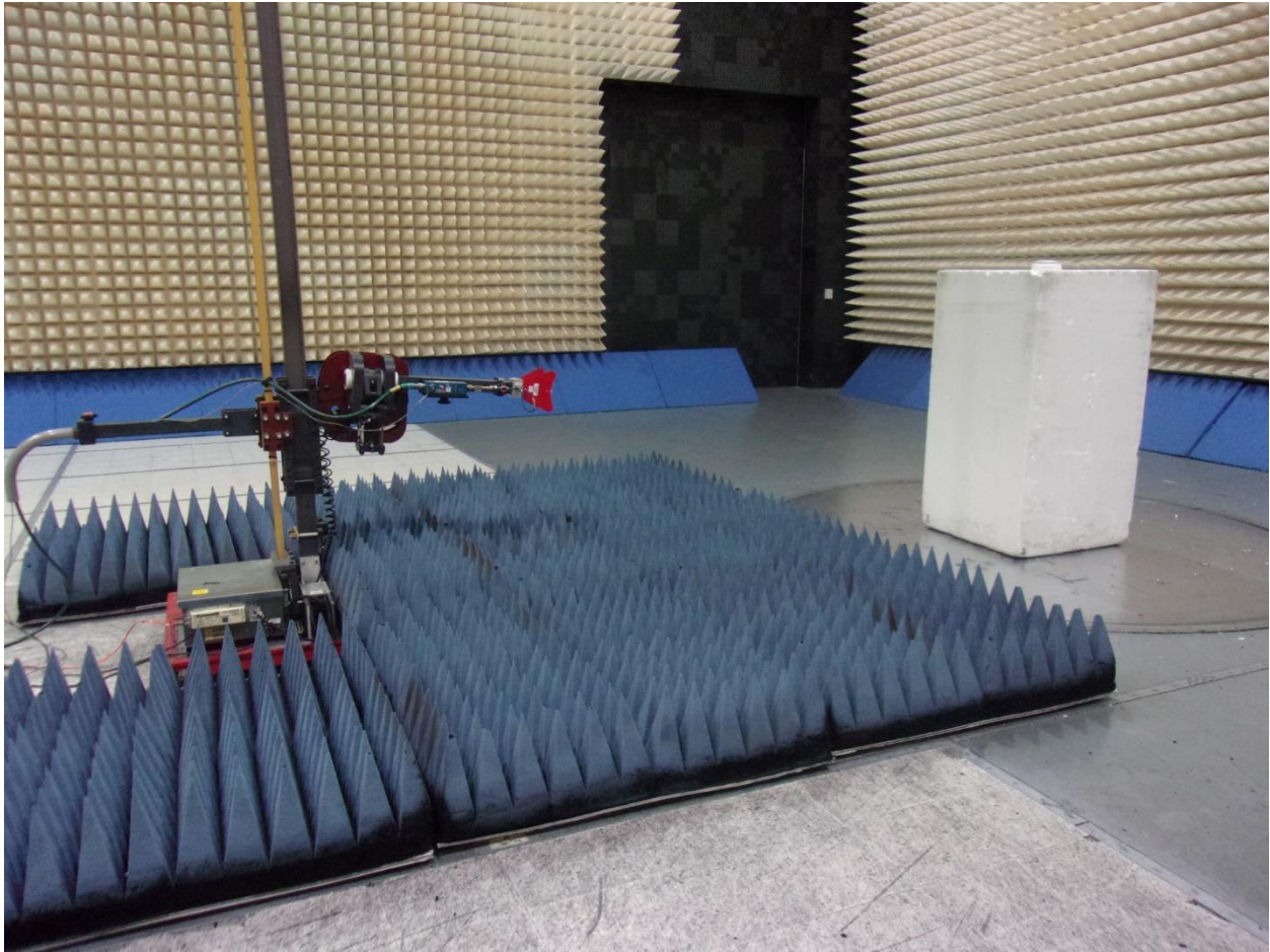
Radiated Emissions: 1GHz-18GHz (Transmitter Active)
