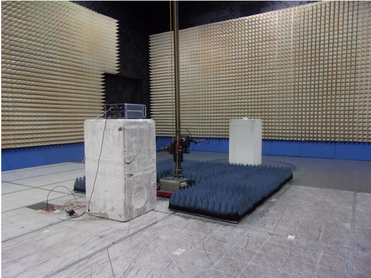
Radiated Emissions: 18GHz-40GHz (Transmitter Active)
