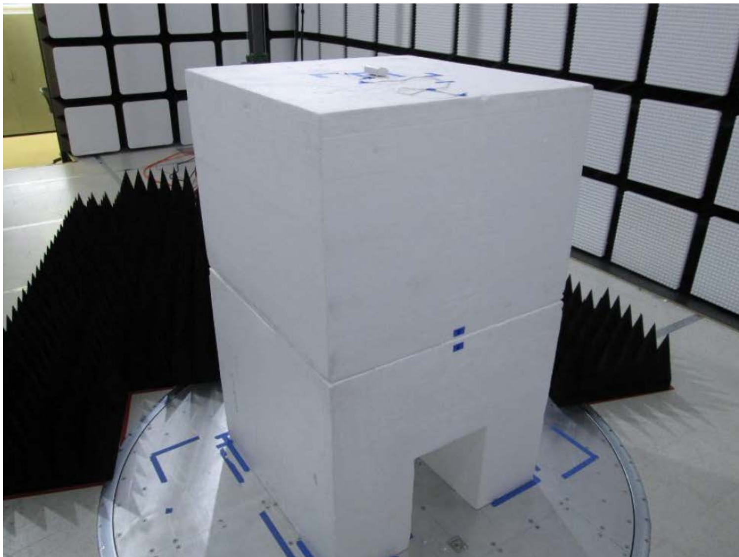
ANT1 Radiated Testing Above 1GHz - Back View
