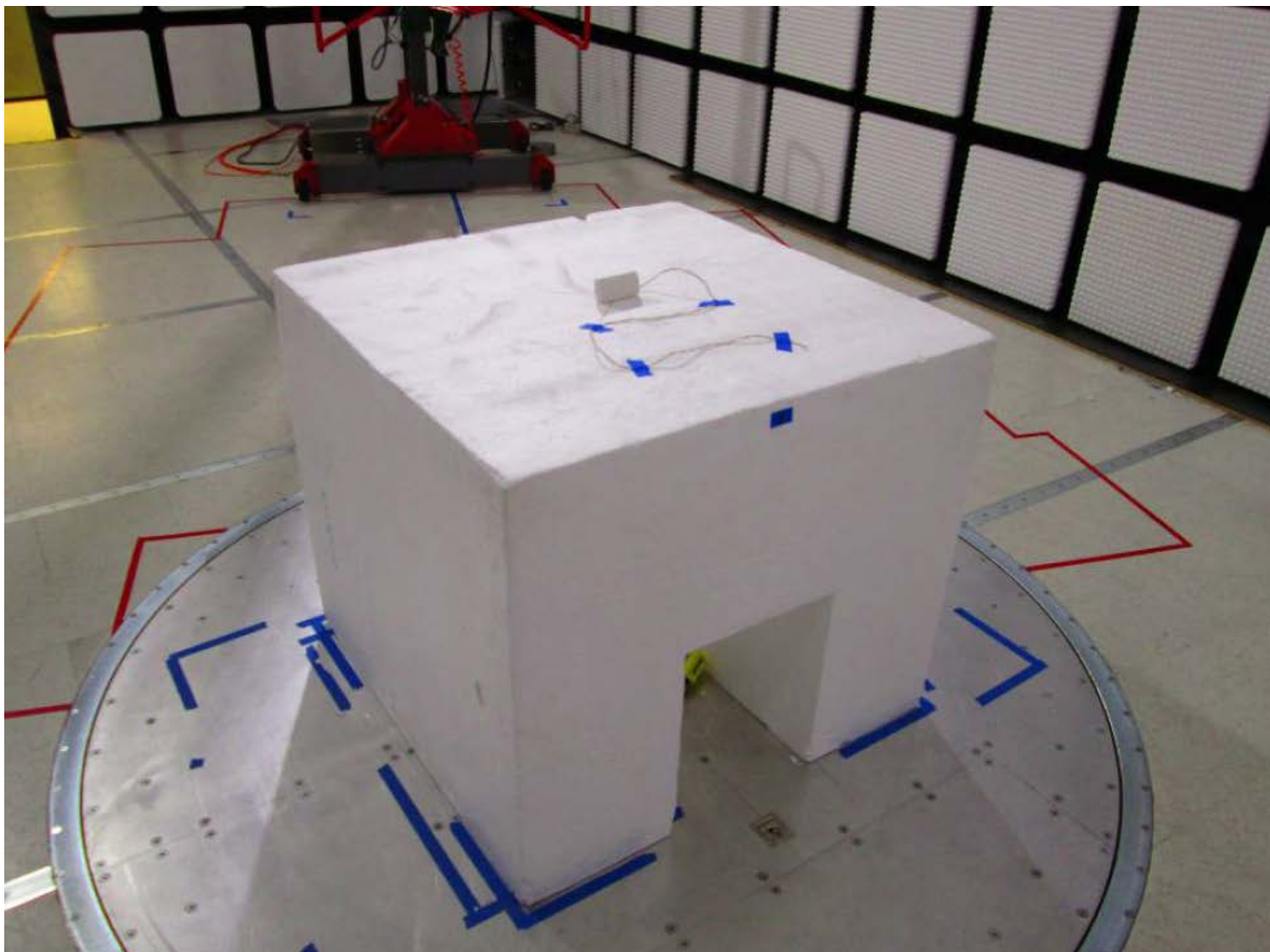
ANT2 Radiated Testing Below 1GHz - Back View
