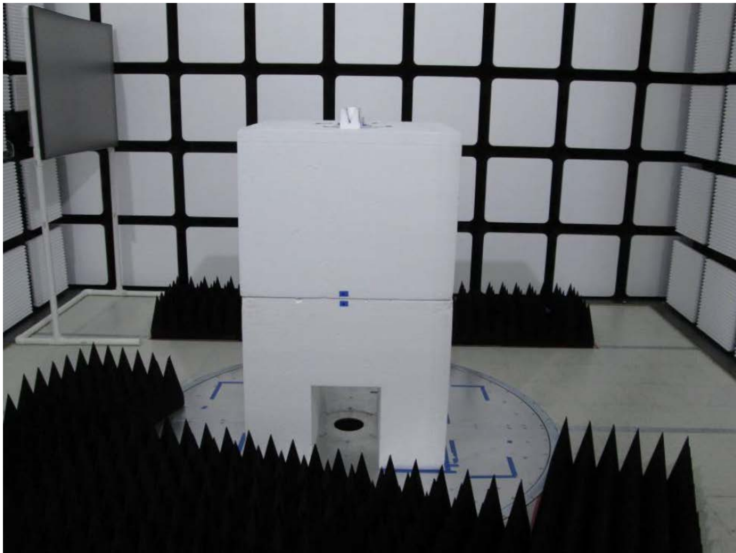
ANT2 Radiated Testing Above 1GHz - Front View
