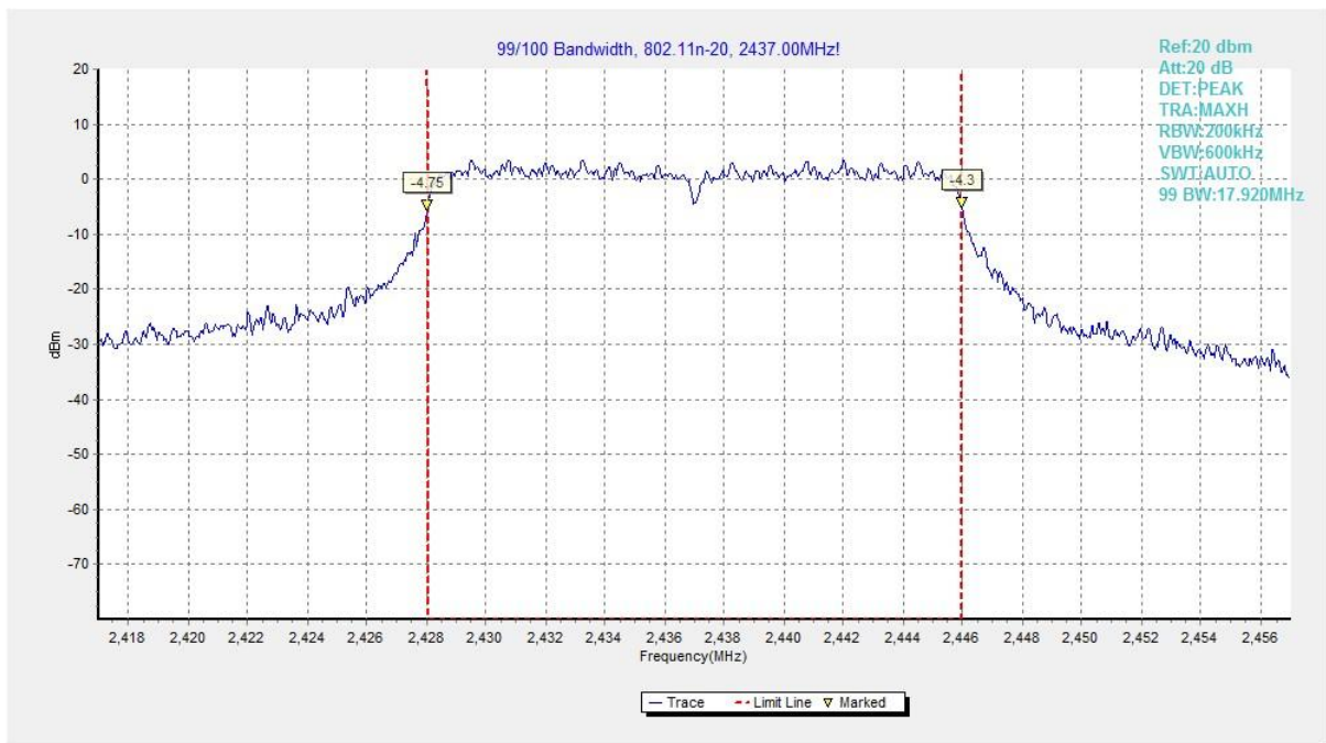
Fig.63 99% Occupied Bandwidth (802.11n HT20, CH 6)
