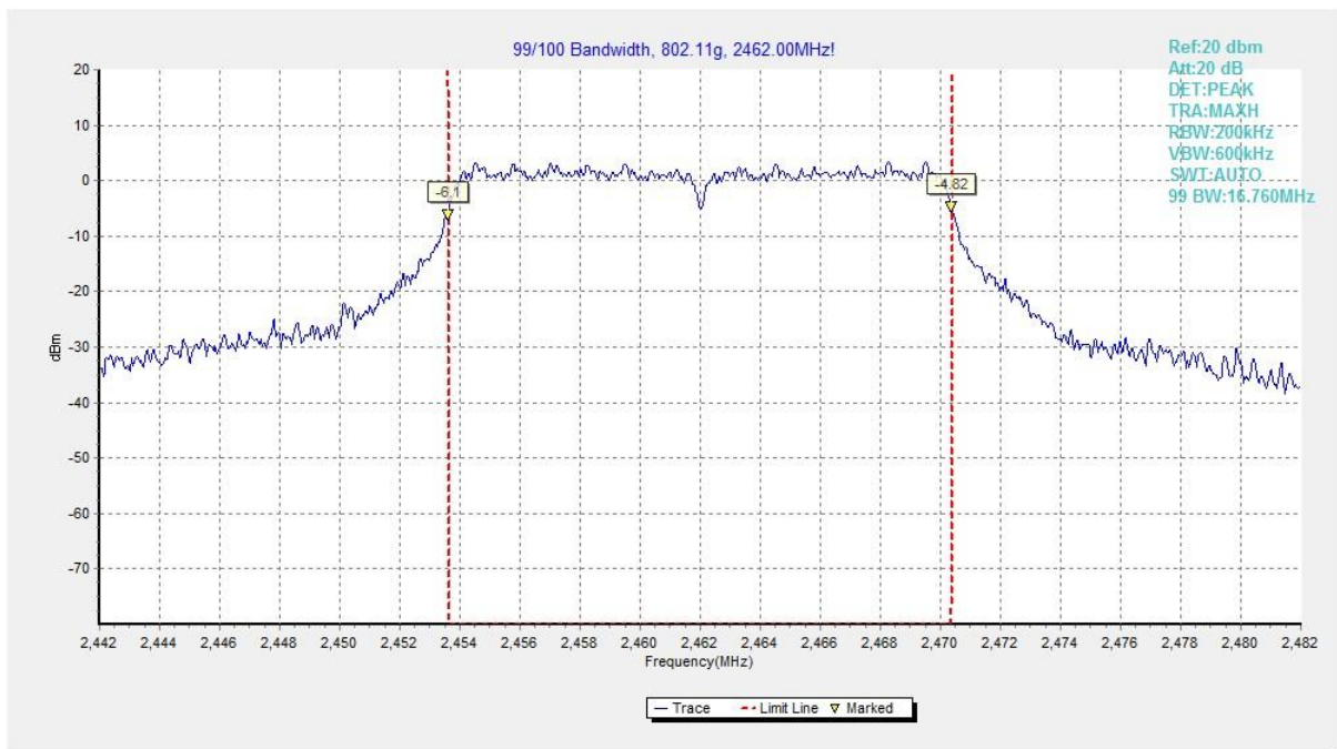
Fig.61 99% Occupied Bandwidth (802.11g, CH 11)
