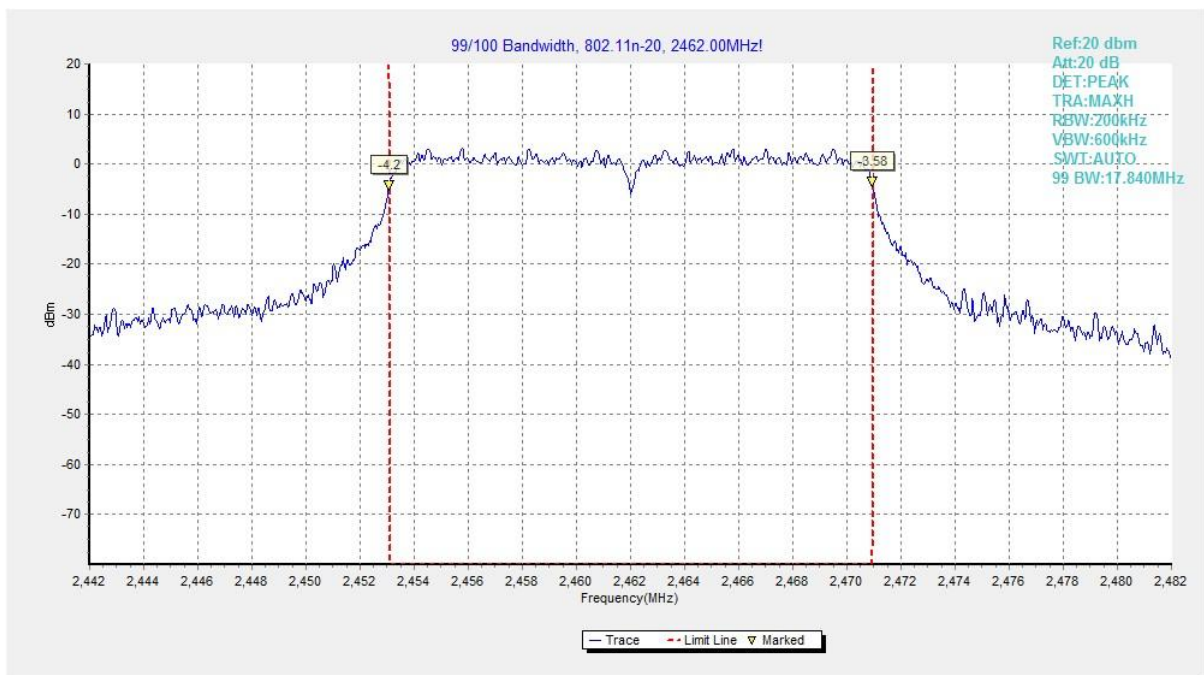
Fig.64 99% Occupied Bandwidth (802.11n HT20, CH 11)
