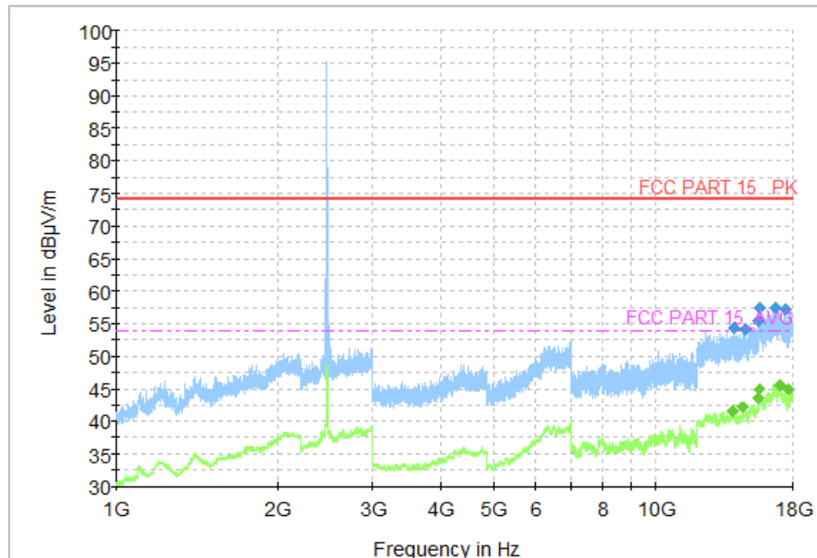
Fig.36 Radiated Spurious Emission (802.11b, CH11, 1GHz-18GHz)
