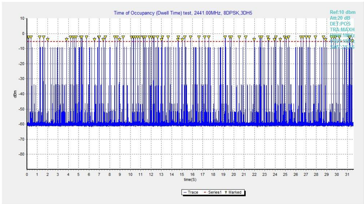
Fig. 74 Number of Transmissions (8DPSK, Ch39)
