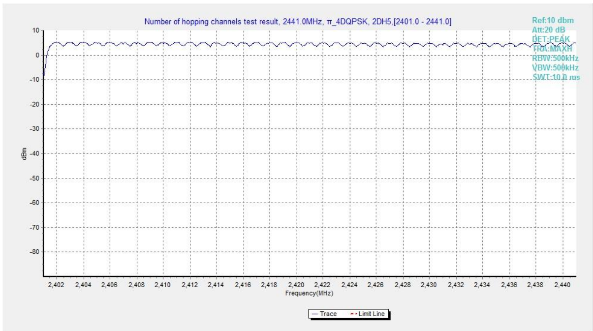
Fig. 77 Hopping channel ch0 ~ ch39 ( \pi/4 DQPSK)
