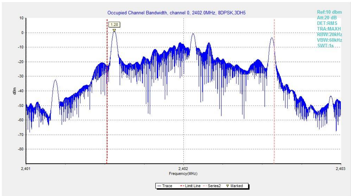
Fig. 94 Occupied Bandwidth (8DPSK, Ch 0)
