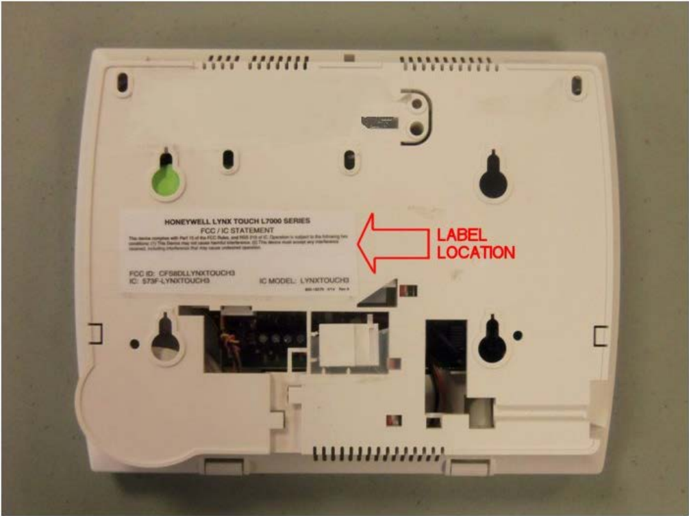
CASE BACK
