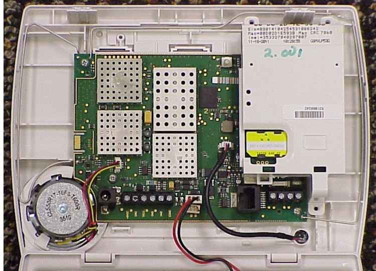
2. LYNXTOUCH2 WITH 3G MODULE:
