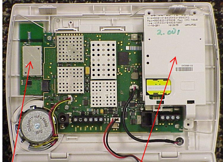
4. LYNXTOUCH2 WITH 3G & WIFI MODULES:
