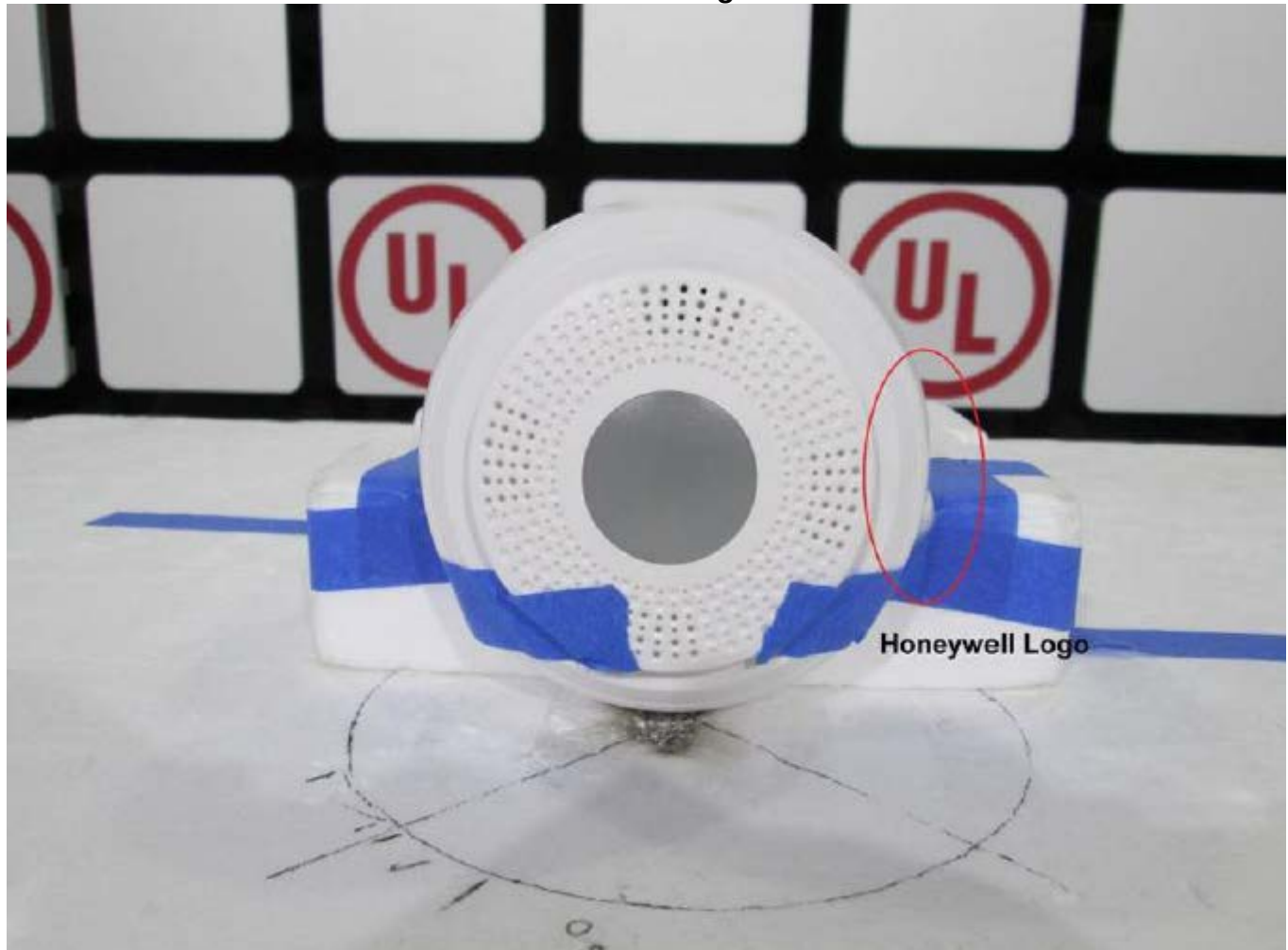
Above 1GHz Testing - Z Axis
