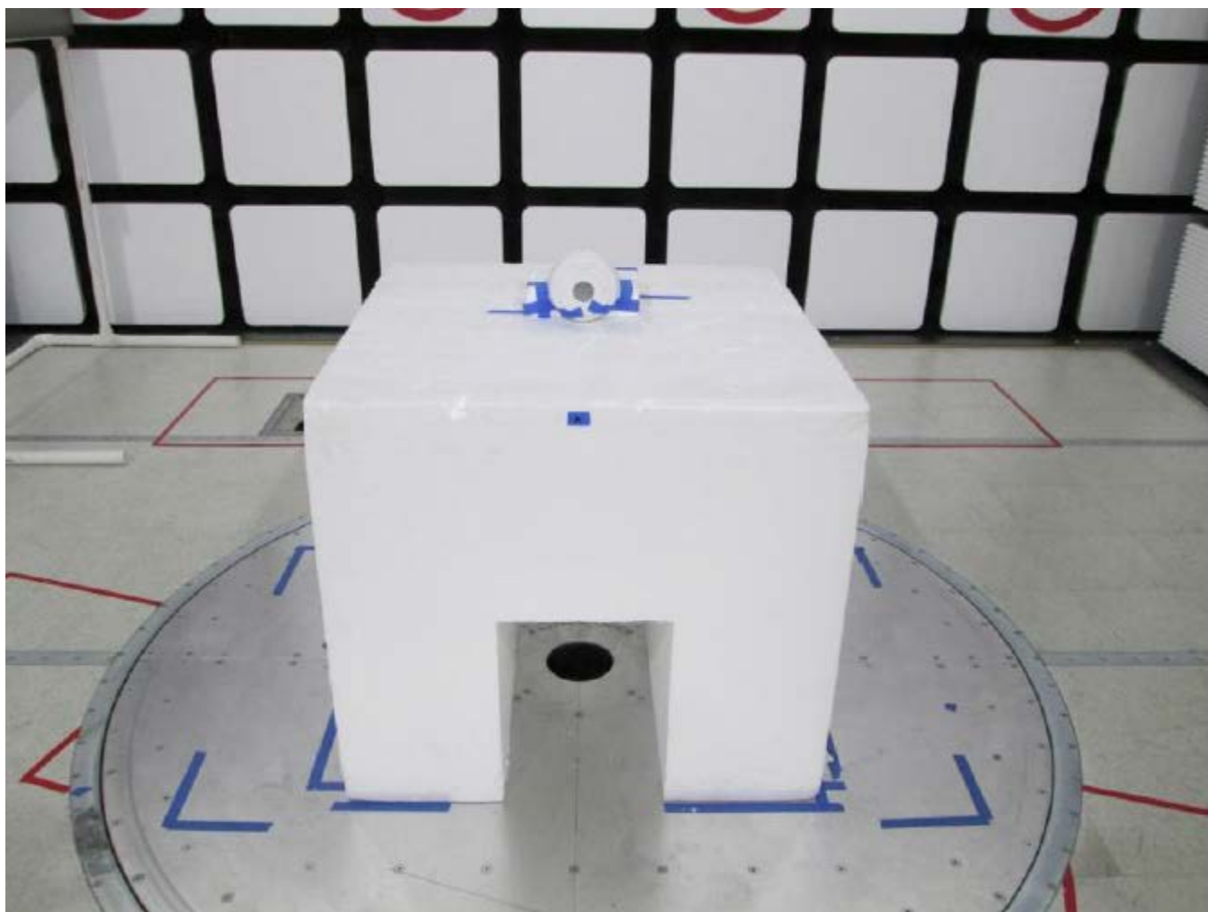
Radiated Testing Below 1GHz - Front View
