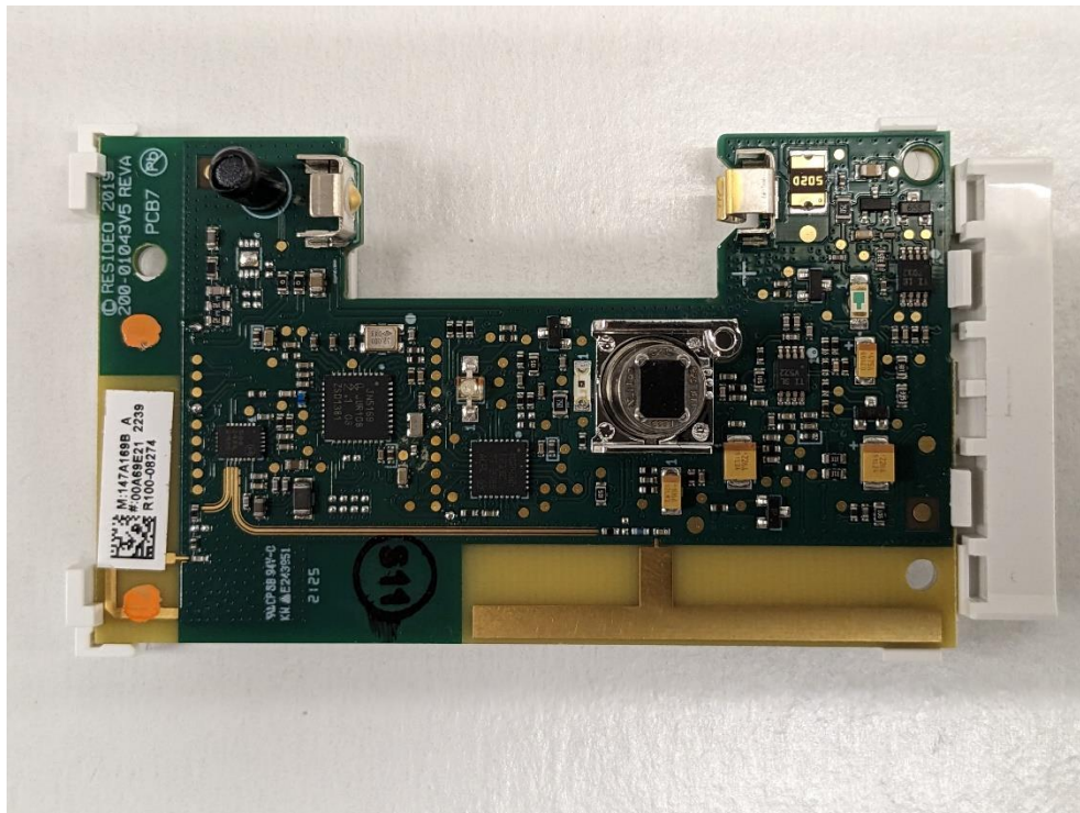
Figure 2 PCB TOP VIEW
