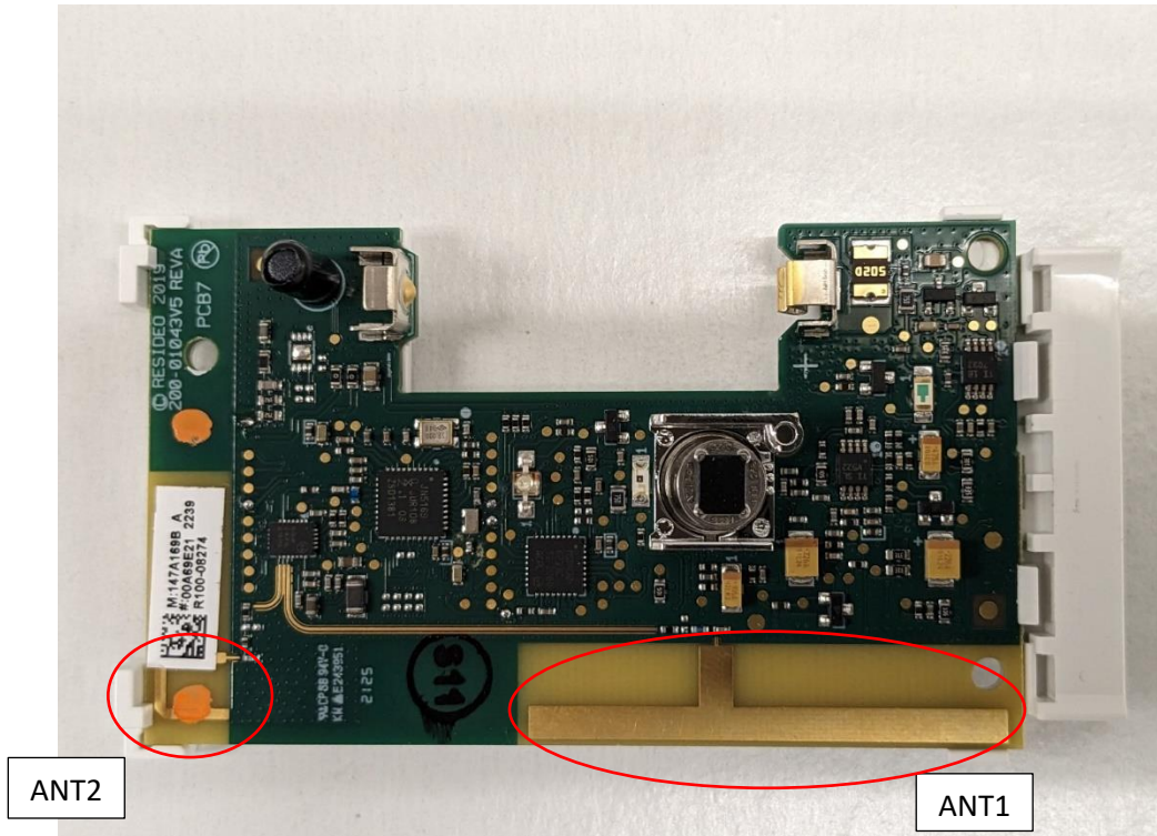
Figure 3 PCB with Antennas
