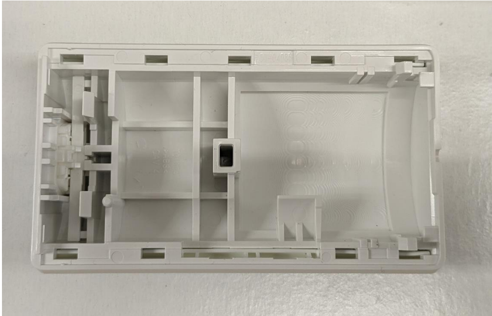
Figure 6 Case Interior Top cover
