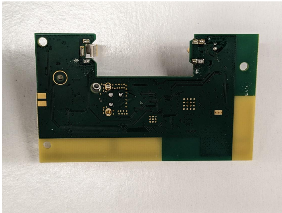
Figure 4 PCB BACK
