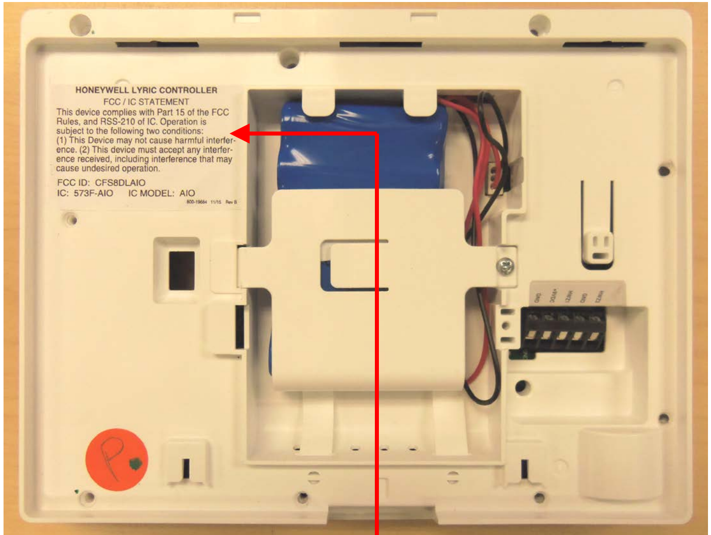
CASE BACK WITH WALL MOUNT BRACKET REMOVED
