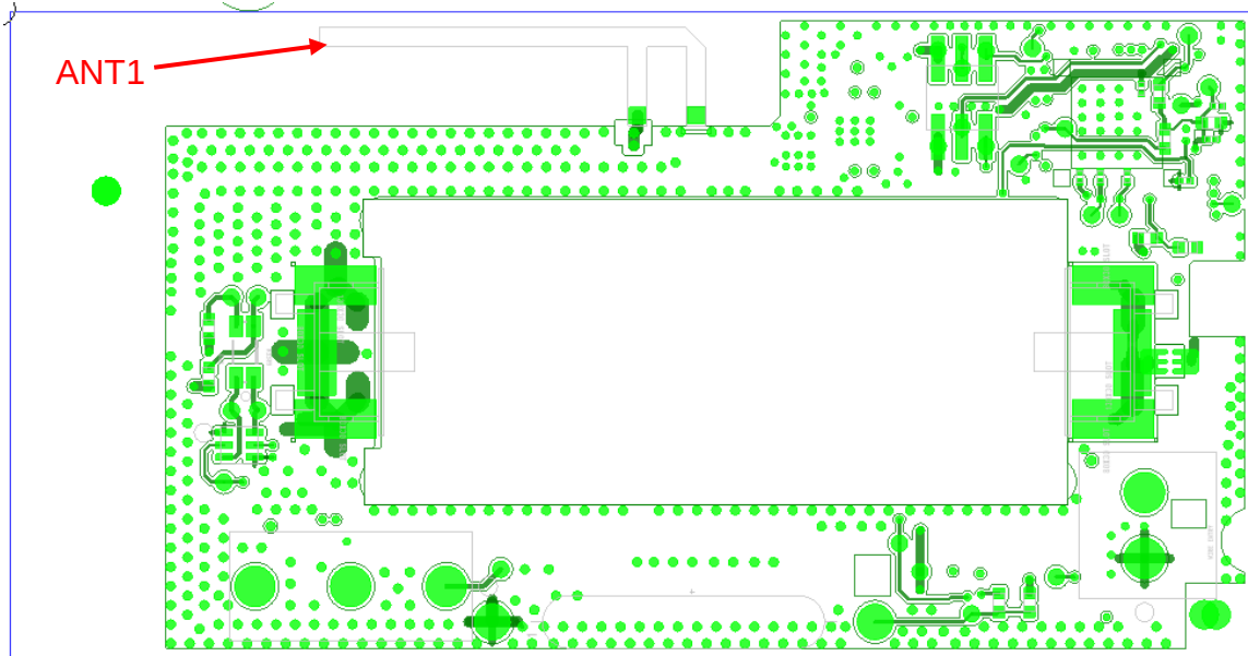
PCB TOP - DRAWING SHOWING ANTENNA 1 LOCATION
