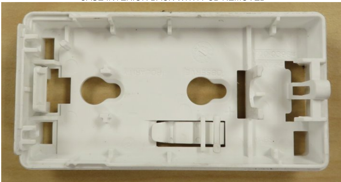
CASE INTERIOR BACK WITH PCB REMOVED
