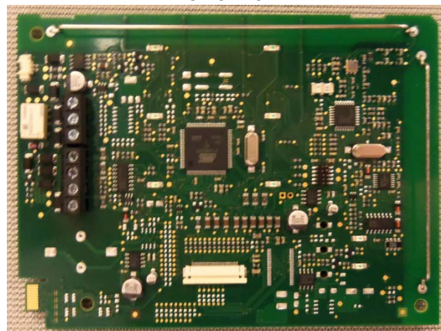
TOP OF PCB
