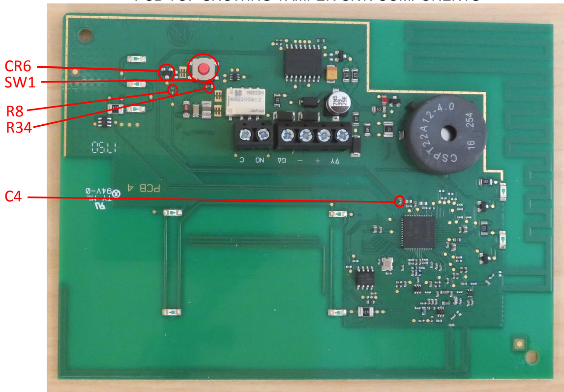
PCB TOP SHOWING TAMPER CKT. COMPONENTS
