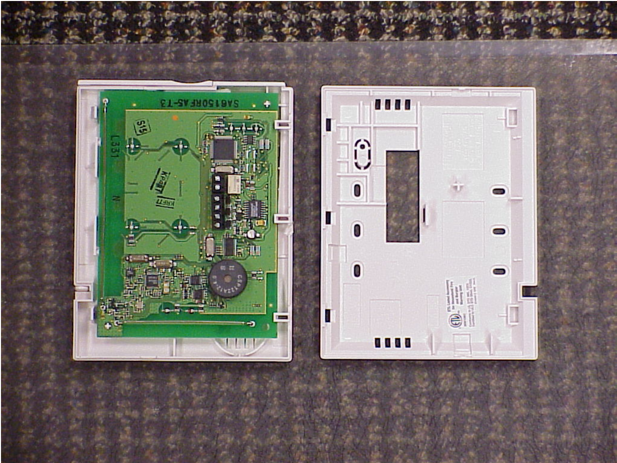
HOW PCB CONTACTS LCD & KEYPAD:
