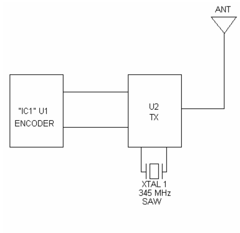
Honeywell 5878 Single Chip Transmitter
