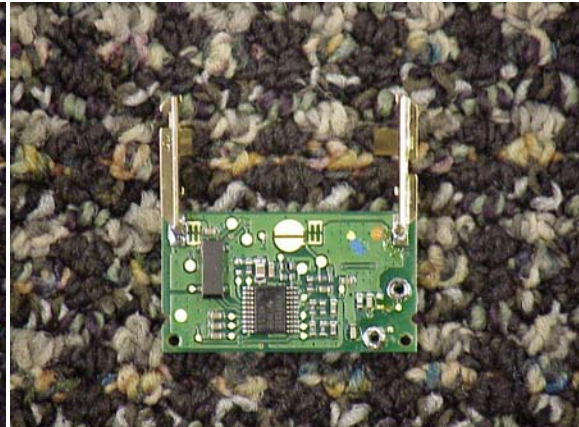
INTERNAL - PCB TOP
