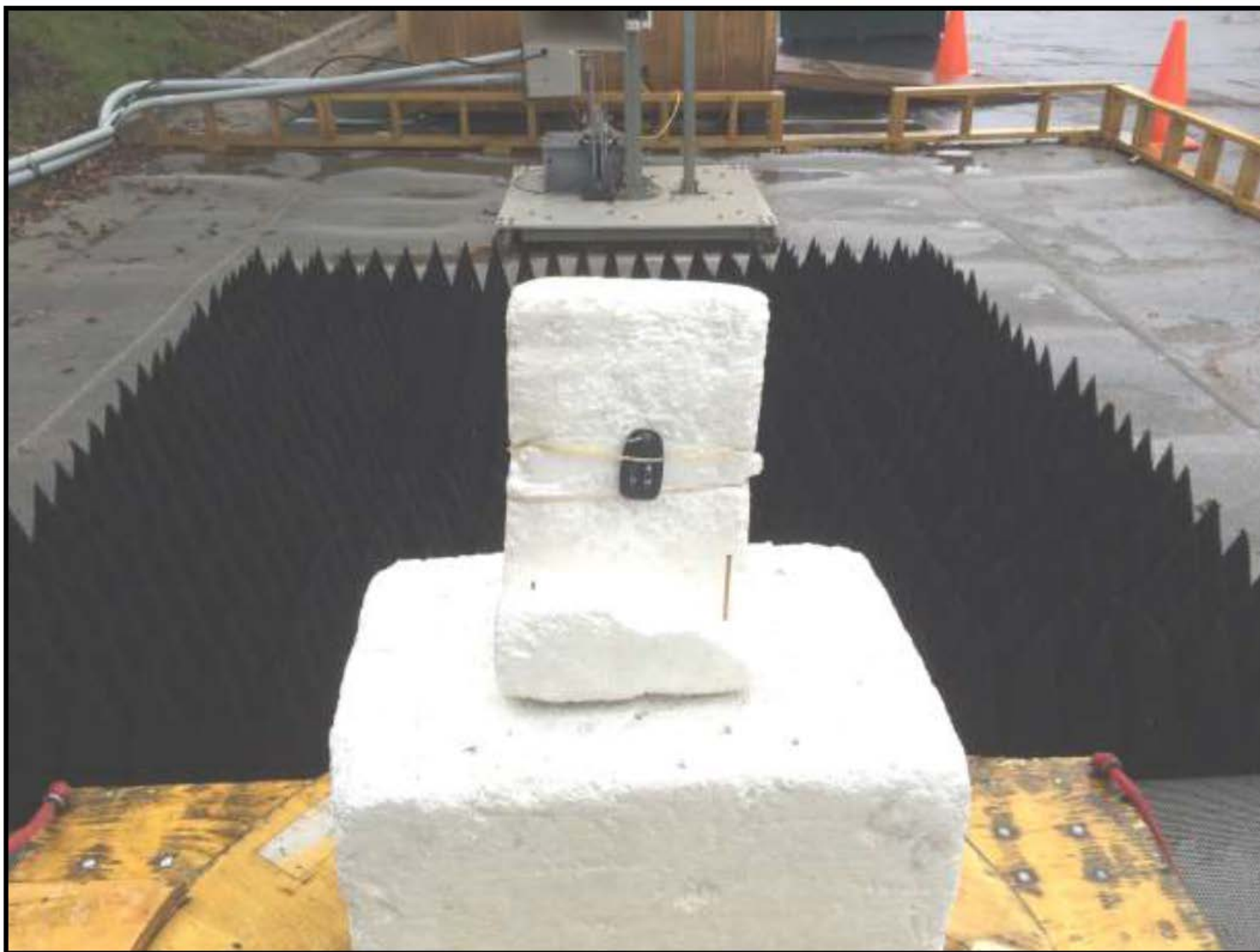
Photograph 1: Radiated Emissions
