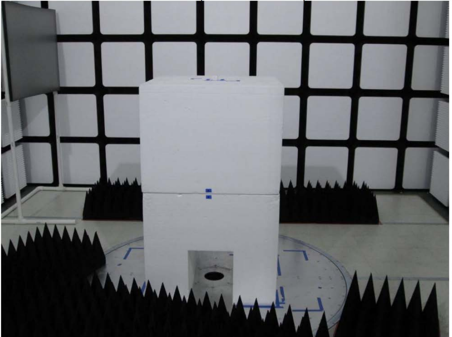
Radiated RF Measurement Setup Above 1GHz - Front View
