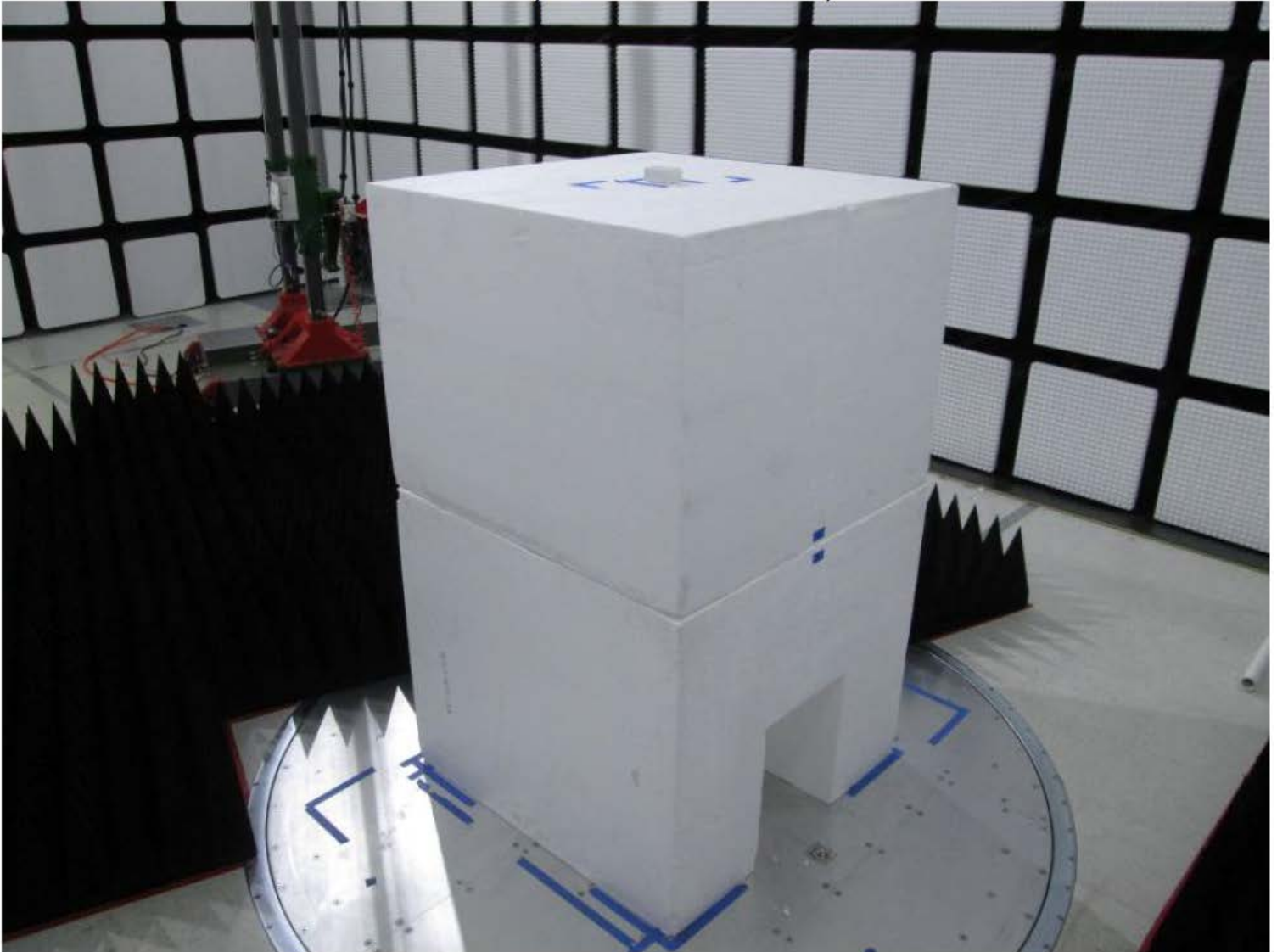
Radiated Testing Above 1GHz - Back View
