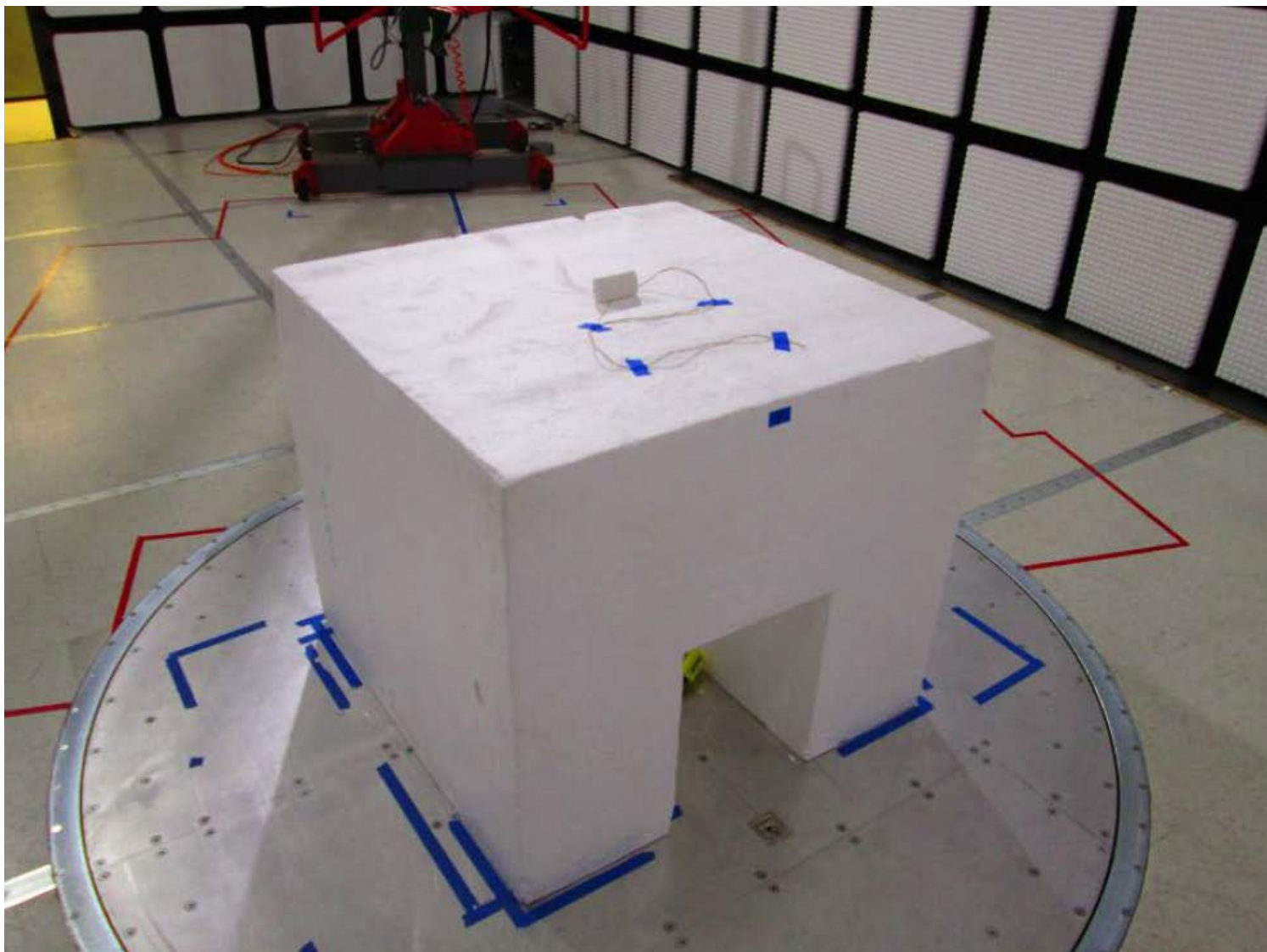
Radiated Testing Below 1GHz - Back View
