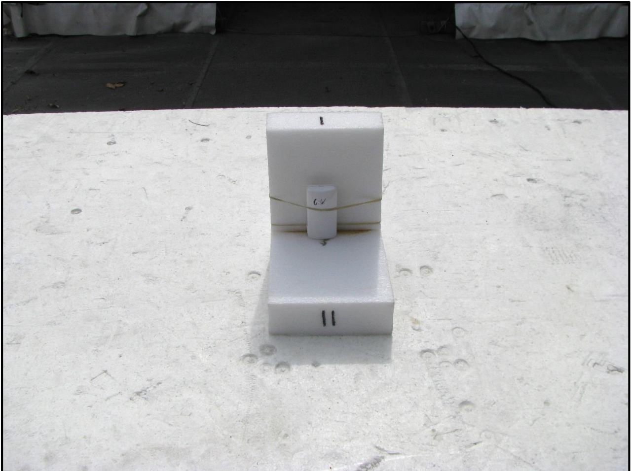
Photograph 1: Radiated Emissions
