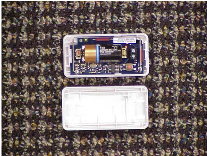
TOP OF THE PCB
