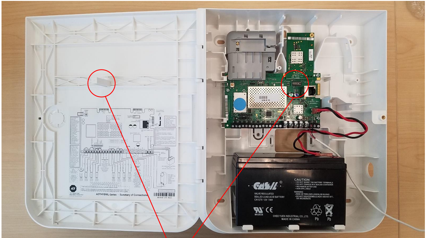
Tamper switch and actuator.
