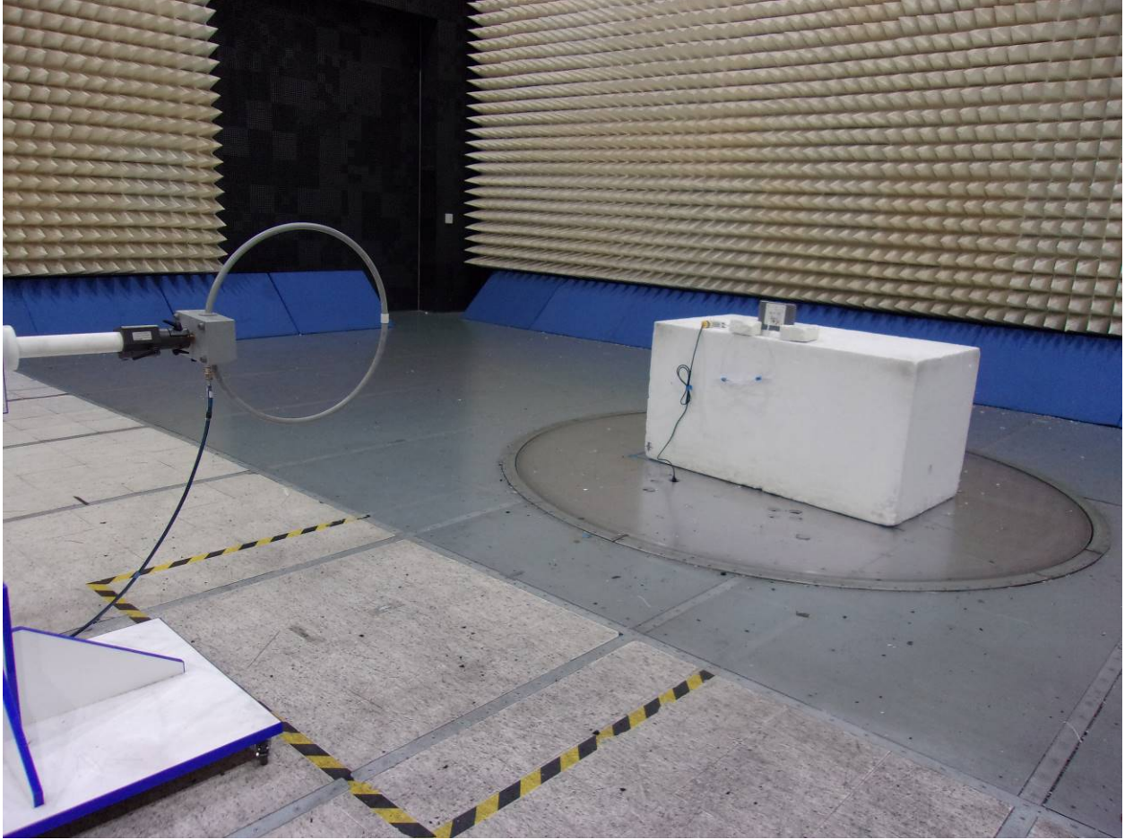
Radiated Spurious Emissions (below 30MHz)
