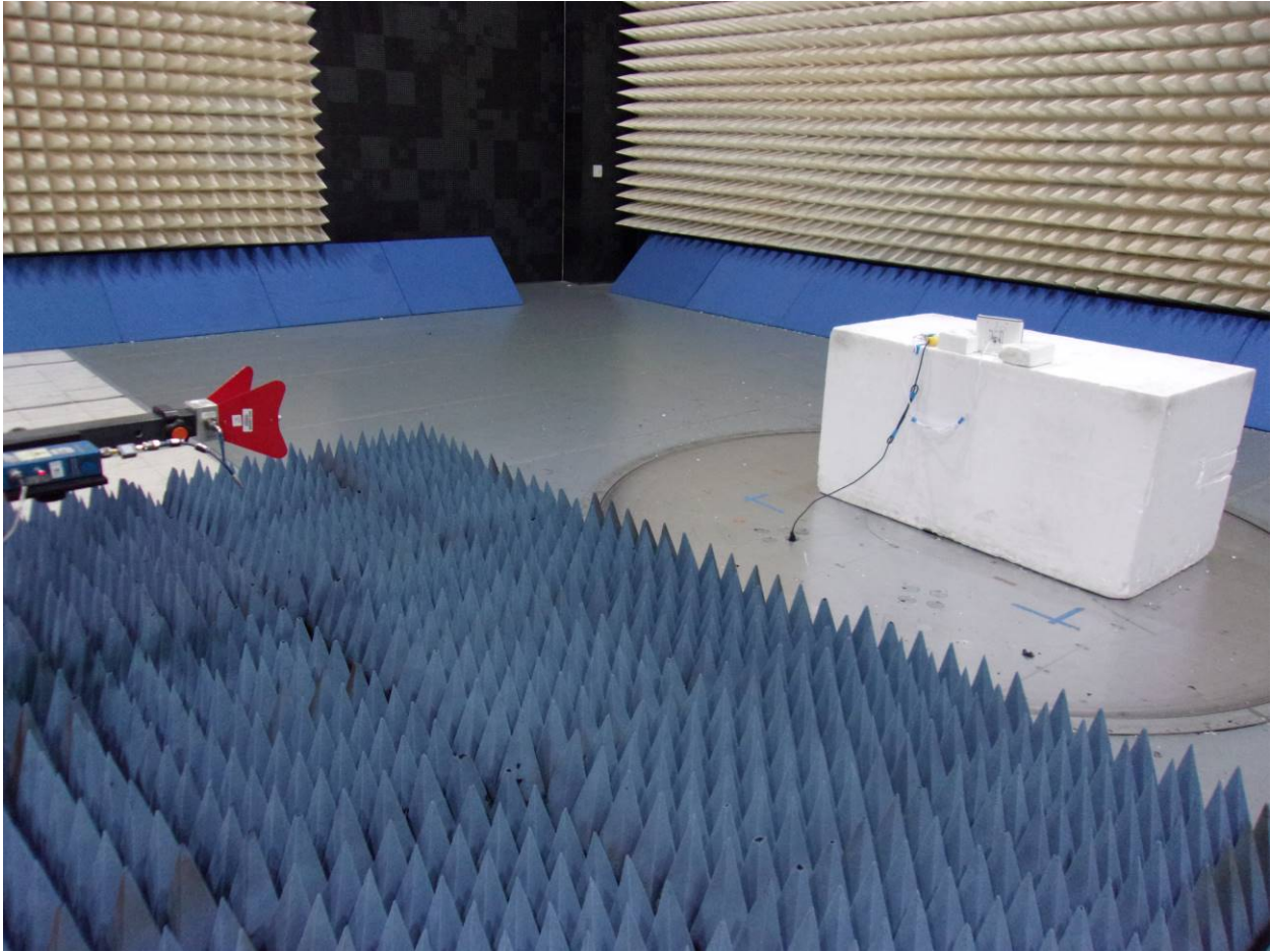
Radiated Digital Device Emissions
