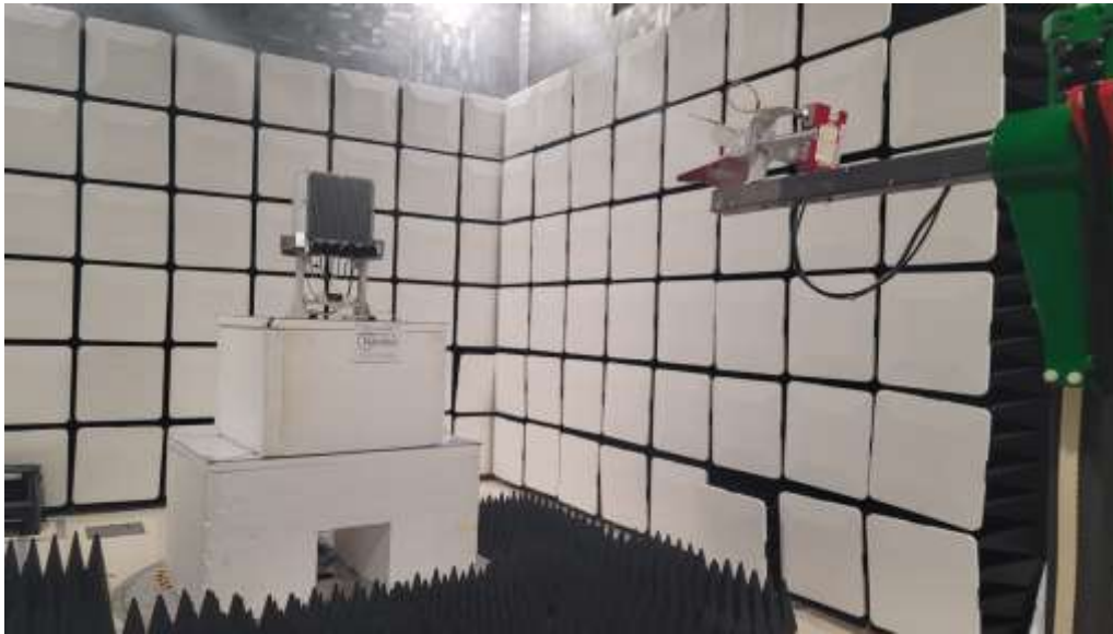
Figure 3 - Radiated emissions above 1 GHz (1 – 7 GHz), front view.
