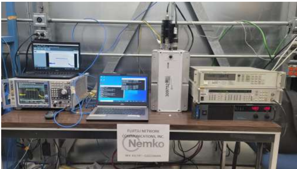
Figure 6 – Test setup (spectrum analyzer measurements)
