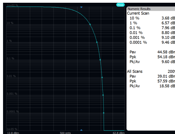
Output Power: Band 71, 256QAM, 20MHz, High Channel, Port A
