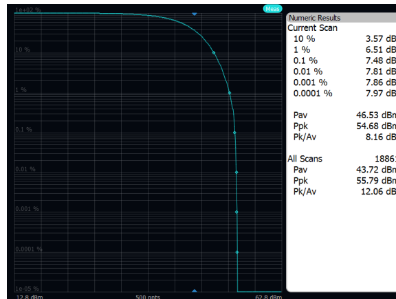
Output Power: Band n29, 64QAM, 10MHz, Mid Channel, Port A
