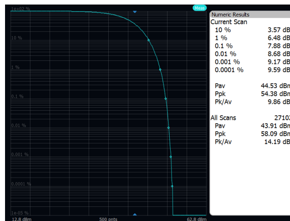
Output Power: Band 71, 64QAM, 20MHz, High Channel, Port A
