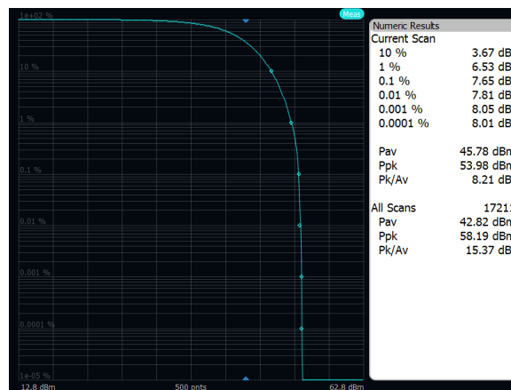
Output Power: Band 71, 16QAM, 5MHz, High Channel, Port A
