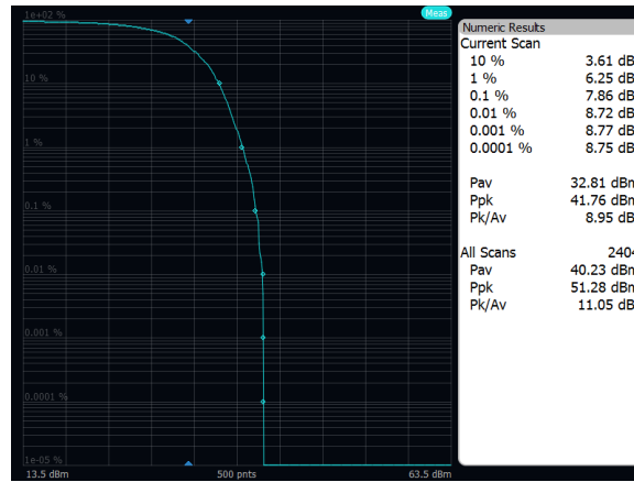
Output Power: Band 26, NBIOT Only (GB) Low Channel, Port A
