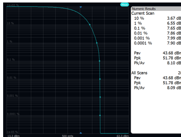
Output Power: Band 71, QPSK, 10MHz, Mid Channel, Port A
