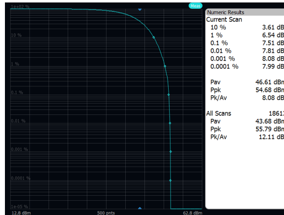
Output Power: Band n29, 64QAM, 10MHz, Low Channel, Port A
