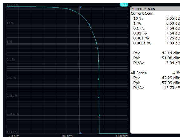
Output Power: Band 71, 256QAM, 5MHz, Mid Channel, Port A
