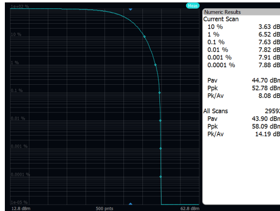
Output Power: Band 71, 64QAM, 5MHz, Low Channel, Port A
