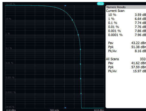
Output Power: Band 71, 256QAM, 10MHz, Mid Channel, Port A
