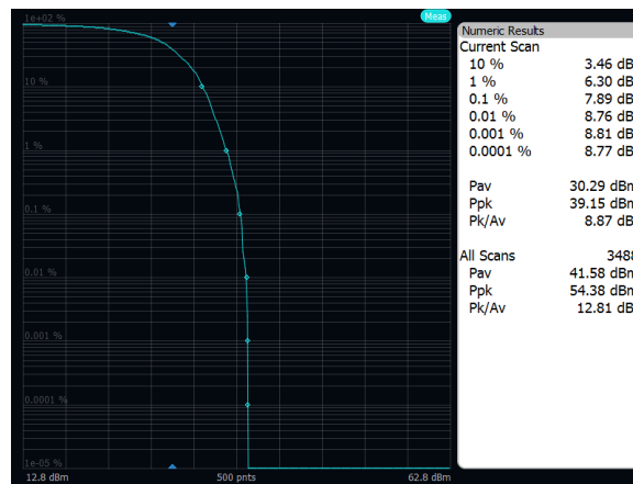
Output Power: Band 71, NBIOT Mid Channel, Standalone
