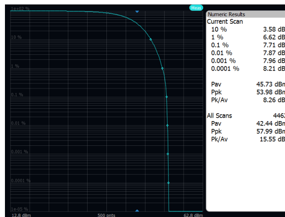
Output Power: Band 71, 256QAM, 5MHz, High Channel, Port A
