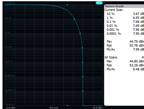
Output Power: Band 71, QPSK, 5MHz, Low Channel, Port A
