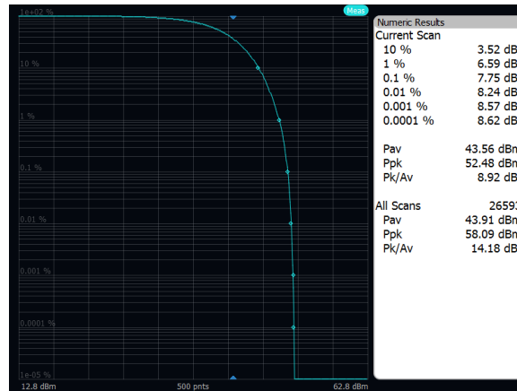
Output Power: Band 71, 64QAM, 20MHz, Low Channel, Port A
