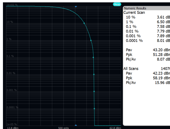
Output Power: Band 71, 16QAM, 10MHz, Mid Channel, Port A
