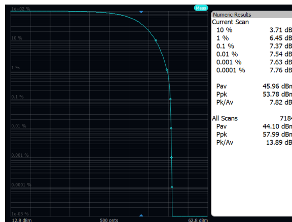
Output Power: Band n29, 256QAM, 5MHz, High Channel, Port A
