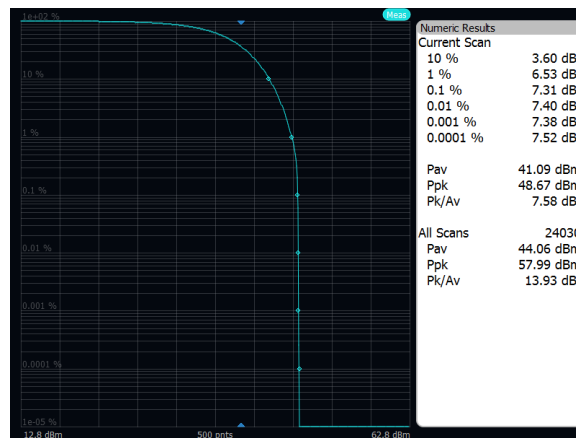
Output Power: Band 26, 64QAM, 5MHz, Mid Channel, Port A
