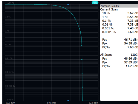
Output Power: Band n29, QPSK, 5MHz, Low Channel, Port A
