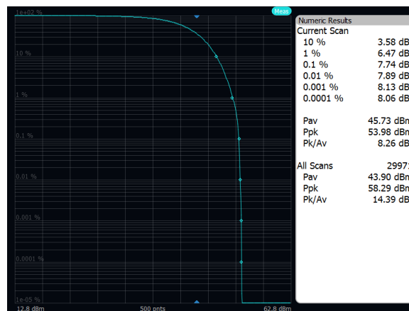
Output Power: Band 71, 64QAM, 5MHz, High Channel, Port A
