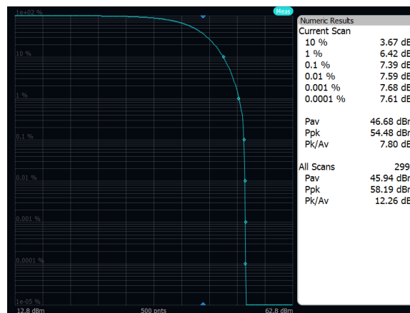
Output Power: Band n29, 16QAM, 5MHz, High Channel, Port A
