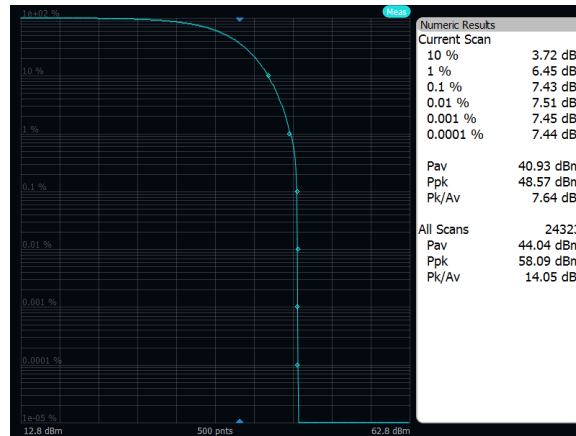
Output Power: Band 26, 64QAM, 5MHz, Low Channel, Port A
