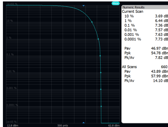
Output Power: Band n29, 256QAM, 5MHz, Low Channel, Port A
