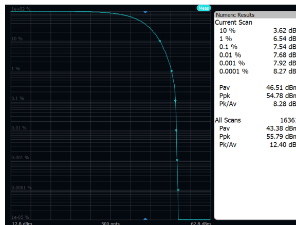
Output Power: Band n29, QPSK, 10MHz, High Channel, Port A
