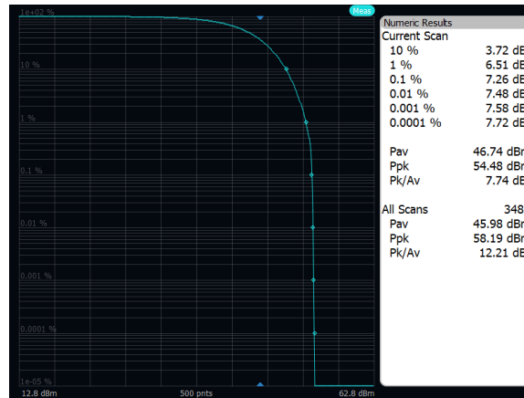
Output Power: Band n29, 16QAM, 5MHz, Low Channel, Port A
