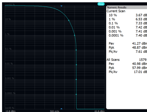
Output Power: Band 26, 256QAM, 5MHz, High Channel, Port A
