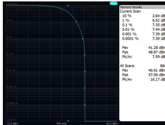
Output Power: Band 26, QPSK, 5MHz, Low Channel, Port A
