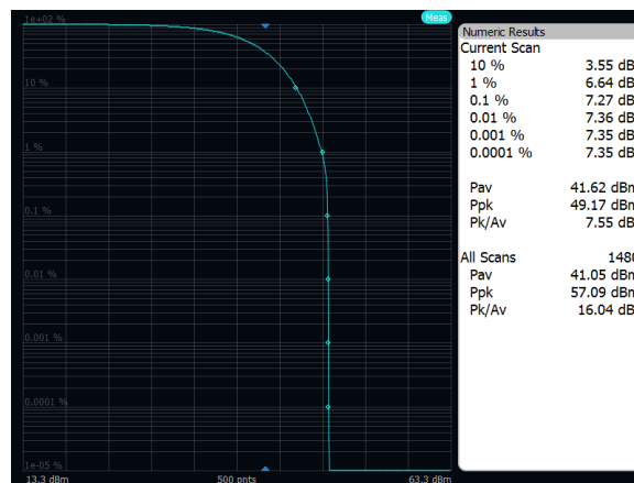
Output Power: Band 26, QPSK, 5MHz, High Channel, Port A
