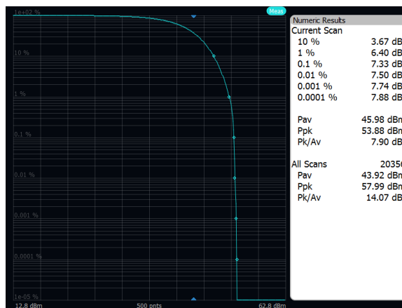
Output Power: Band n29, 64QAM, 5MHz, High Channel, Port A
