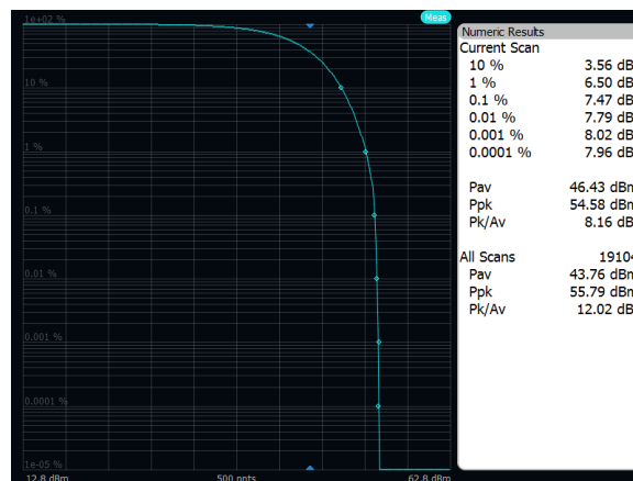
Output Power: Band n29, 64QAM, 10MHz, High Channel, Port A
