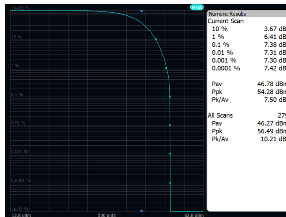
Output Power: Band n29, QPSK, 5MHz, Mid Channel, Port A
