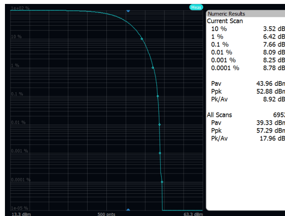
Output Power: Band 71, QPSK, 20MHz, Mid Channel, Port A
