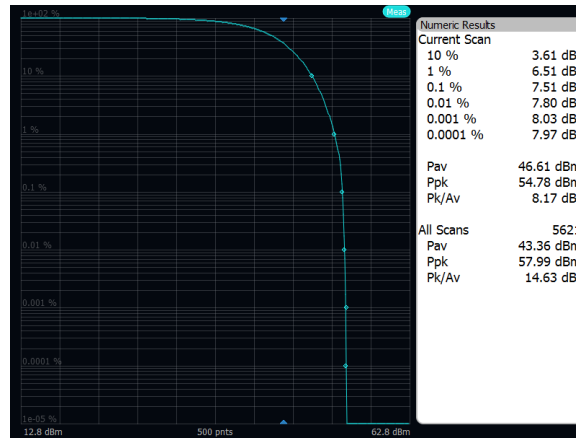
Output Power: Band n29, 256QAM, 10MHz, Low Channel, Port A
