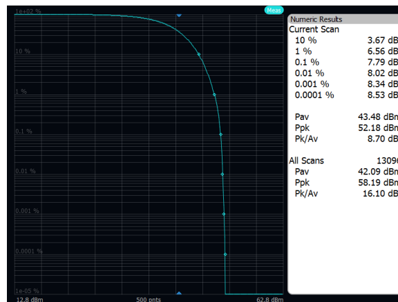
Output Power: Band 71, 16QAM, 20MHz, Mid Channel, Port A
