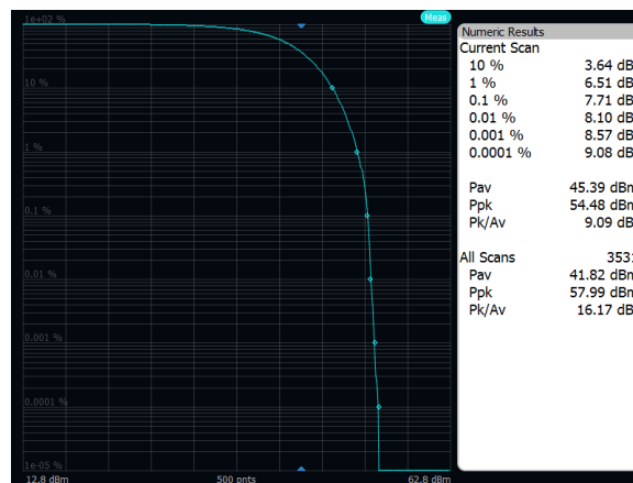
Output Power: Band 71, 256QAM, 10MHz, High Channel, Port A
