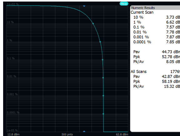
Output Power: Band 71, 16QAM, 5MHz, Low Channel, Port A
