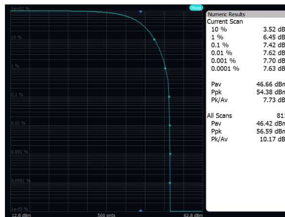
Output Power: Band n29, QPSK, 5MHz, High Channel, Port A
