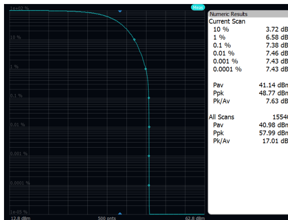
Output Power: Band 26, 256QAM, 5MHz, Mid Channel, Port A
