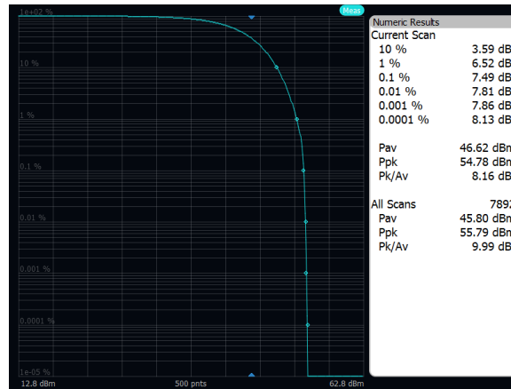
Output Power: Band n29, 16QAM, 10MHz, Low Channel, Port A
