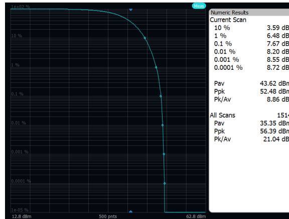
Output Power: Band 71, 256QAM, 20MHz, Low Channel, Port A
