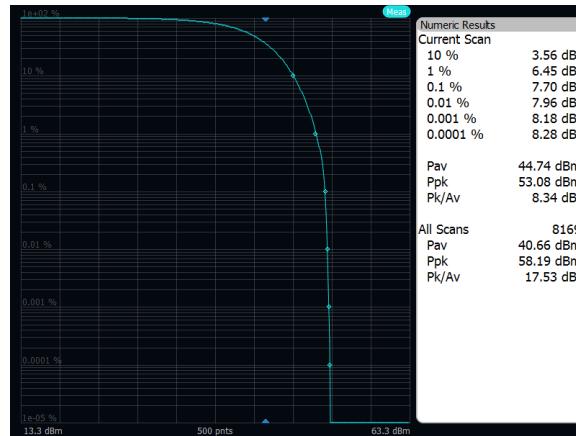
Output Power: Band 71, QPSK, 10MHz, Low Channel, Port A
