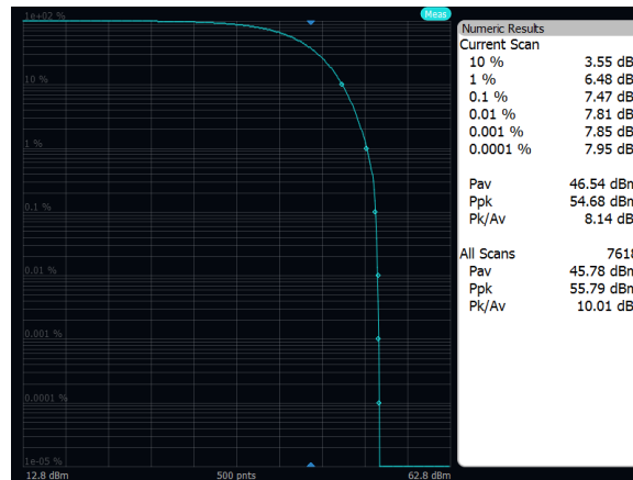
Output Power: Band n29, 16QAM, 10MHz, Mid Channel, Port A
