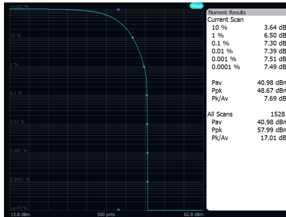
Output Power: Band 26, 256QAM, 5MHz, Low Channel, Port A
