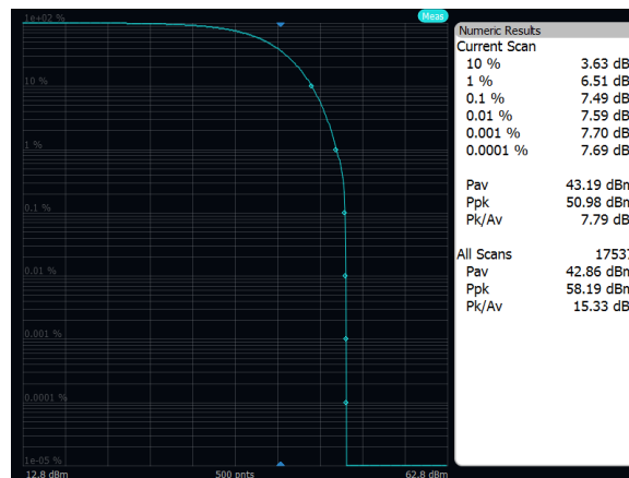
Output Power: Band 71, 16QAM, 5MHz, Mid Channel, Port A
