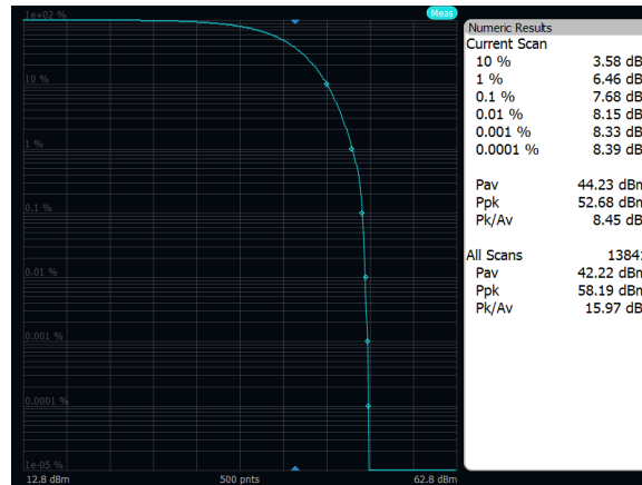
Output Power: Band 71, 16QAM, 10MHz, Low Channel, Port A
