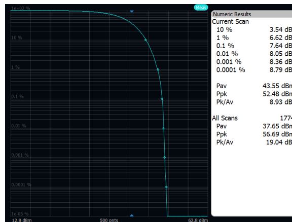
Output Power: Band 71, 256QAM, 20MHz, Mid Channel, Port A
