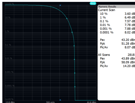
Output Power: Band 71, 64QAM, 10MHz, Mid Channel, Port A
