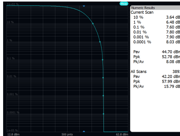
Output Power: Band 71, 256QAM, 5MHz, Low Channel, Port A
