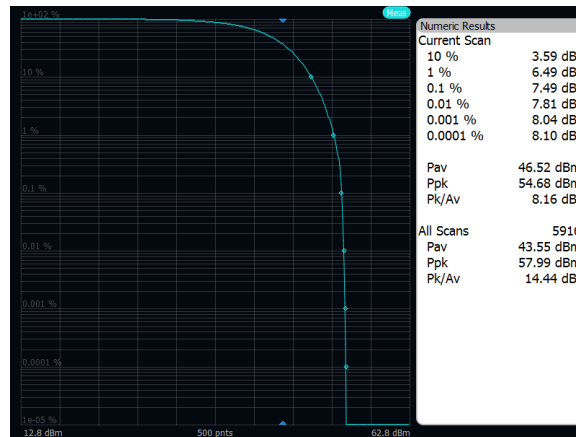
Output Power: Band n29, 256QAM, 10MHz, Mid Channel, Port A
