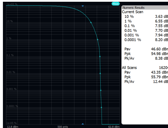
Output Power: Band n29, QPSK, 10MHz, Mid Channel, Port A
