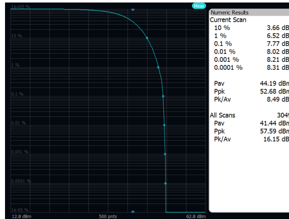
Output Power: Band 71, 256QAM, 10M MHz, Low Channel, Port A
