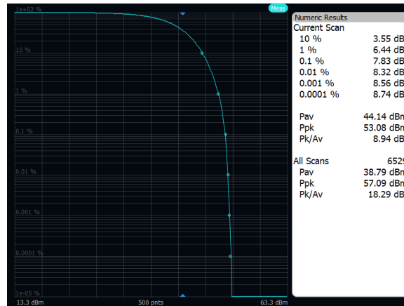
Output Power: Band 71, QPSK, 20MHz, Low Channel, Port A
