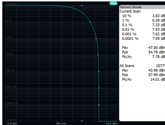
Output Power: Band n29, 64QAM, 5MHz, Low Channel, Port A
