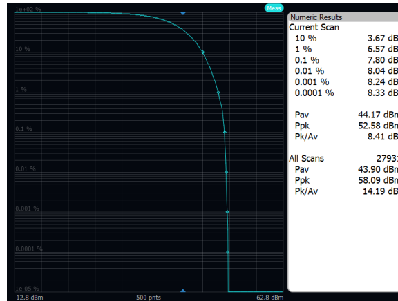
Output Power: Band 71, 64QAM, 10MHz, Low Channel, Port A
