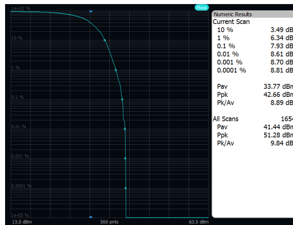
Output Power: Band 26, NBIOT Only (GB) High Channel, Port A
