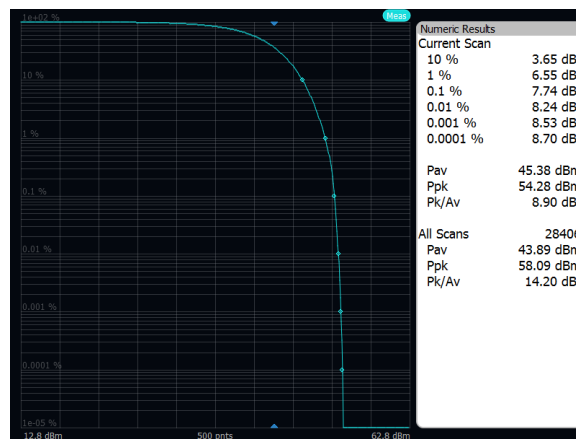
Output Power: Band 71, 64QAM, 10MHz, High Channel, Port A
