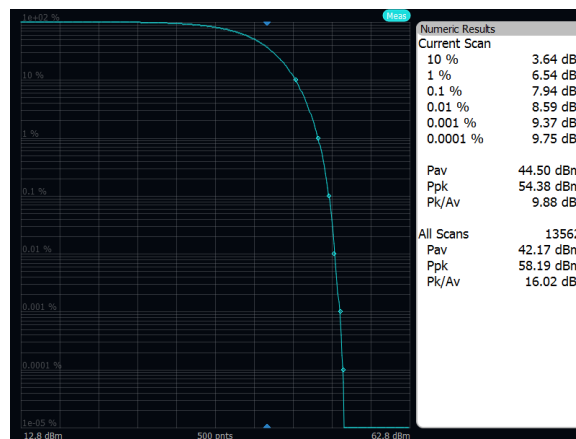
Output Power: Band 71, 16QAM, 20MHz, High Channel, Port A
