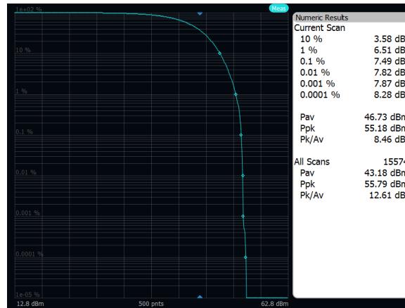
Output Power: Band n29, QPSK, 10MHz, Low Channel, Port A
