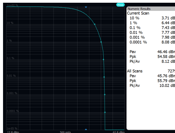
Output Power: Band n29, 16QAM, 10MHz, High Channel, Port A
