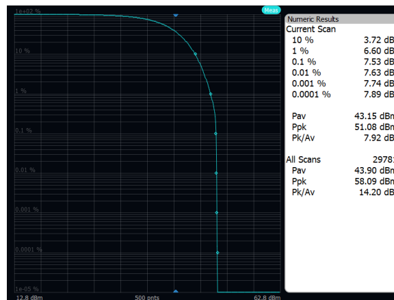
Output Power: Band 71, 64QAM, 5MHz, Mid Channel, Port A
