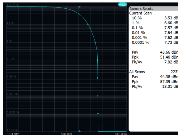
Output Power: Band 71, QPSK, 5MHz, Mid Channel, Port A
