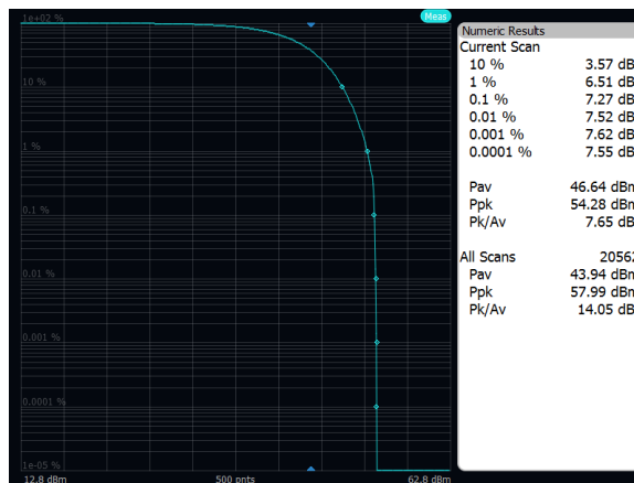
Output Power: Band n29, 64QAM, 5MHz, Mid Channel, Port A
