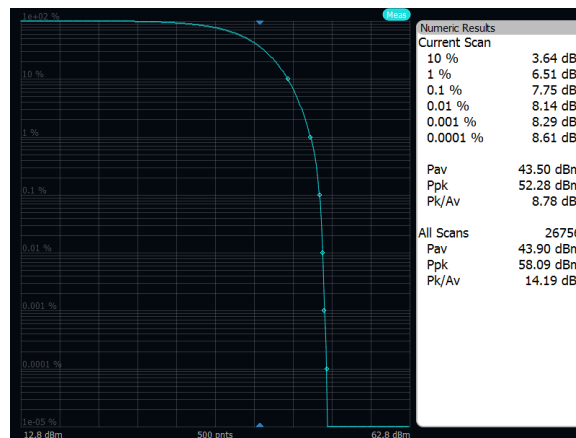
Output Power: Band 71, 64QAM, 20MHz, Mid Channel, Port A
