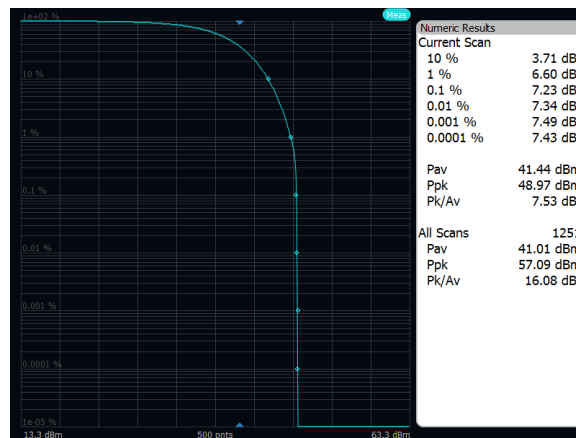
Output Power: Band 26, QPSK, 5MHz, Mid Channel, Port A
