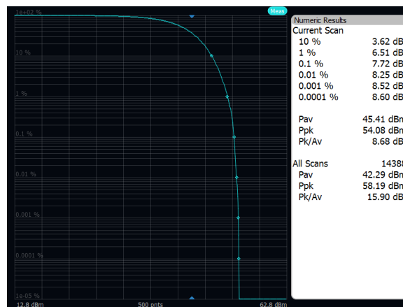
Output Power: Band 71, 16QAM, 10MHz, High Channel, Port A
