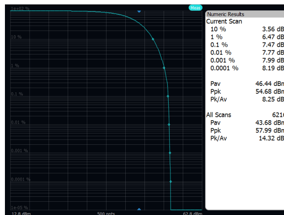
Output Power: Band n29, 256QAM, 10MHz, High Channel, Port A
