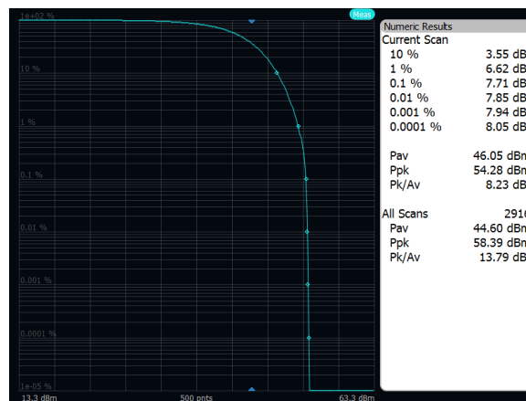
Output Power: Band 71, QPSK, 5MHz, High Channel, Port A
