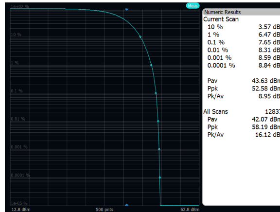
Output Power: Band 71, 16QAM, 20MHz, Low Channel, Port A
