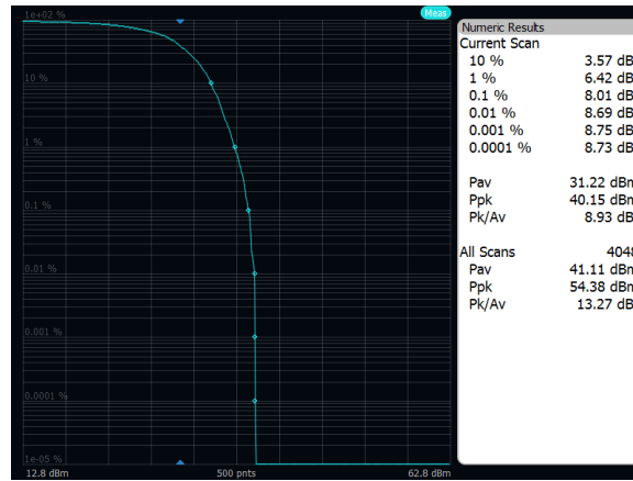
Output Power: Band 71, NBIOT Low Channel, Standalone
