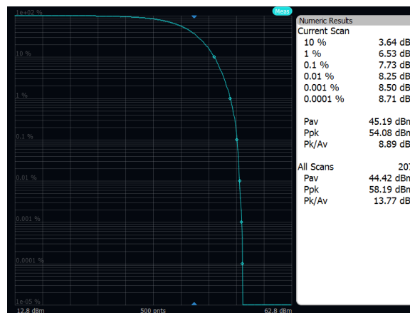
Output Power: Band 71, QPSK, 10MHz, High Channel, Port A
