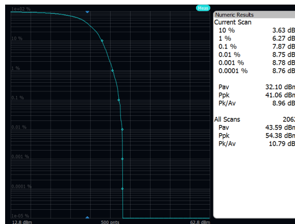
Output Power: Band 71, NBIOT High Channel, Standalone
