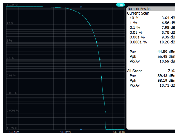
Output Power: Band 71, QPSK, 20MHz, High Channel, Port A
