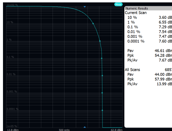
Output Power: Band n29, 256QAM, 5MHz, Mid Channel, Port A
