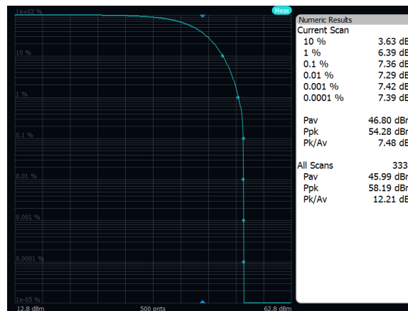
Output Power: Band n29, 16QAM, 5MHz, Mid Channel, Port A
