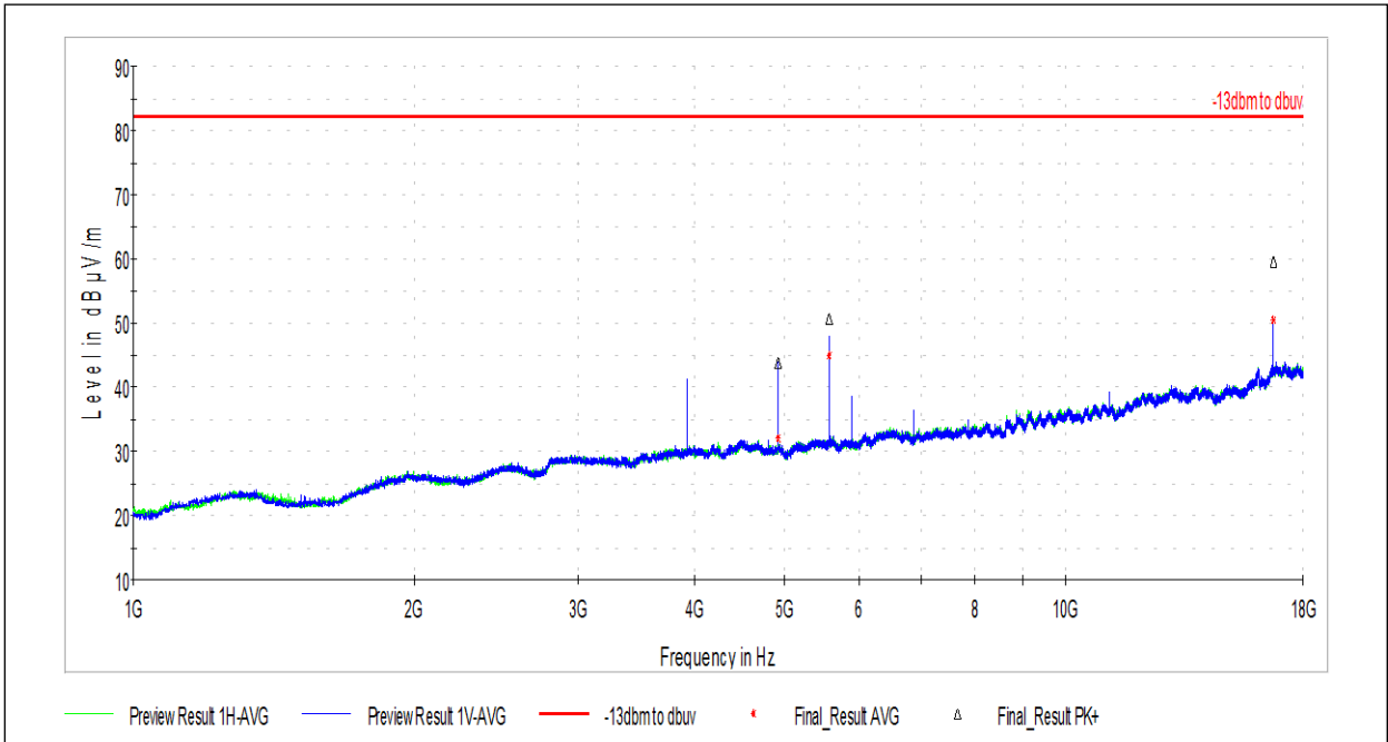
Band n66 High Channel
