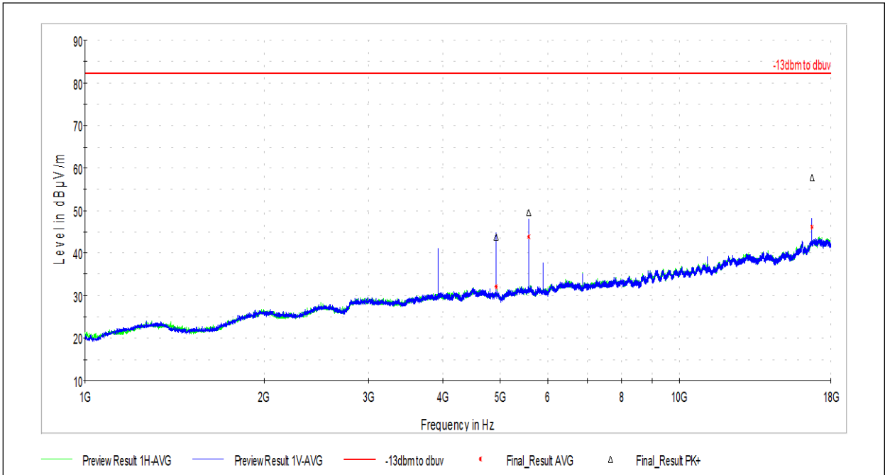
Band n70 Low Channel
