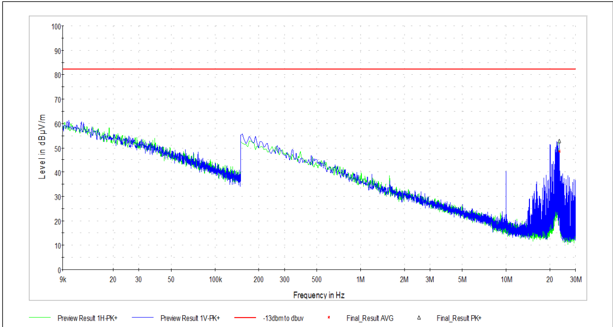
9kHz – 30MHz Scan (valid for all transmit modes)
