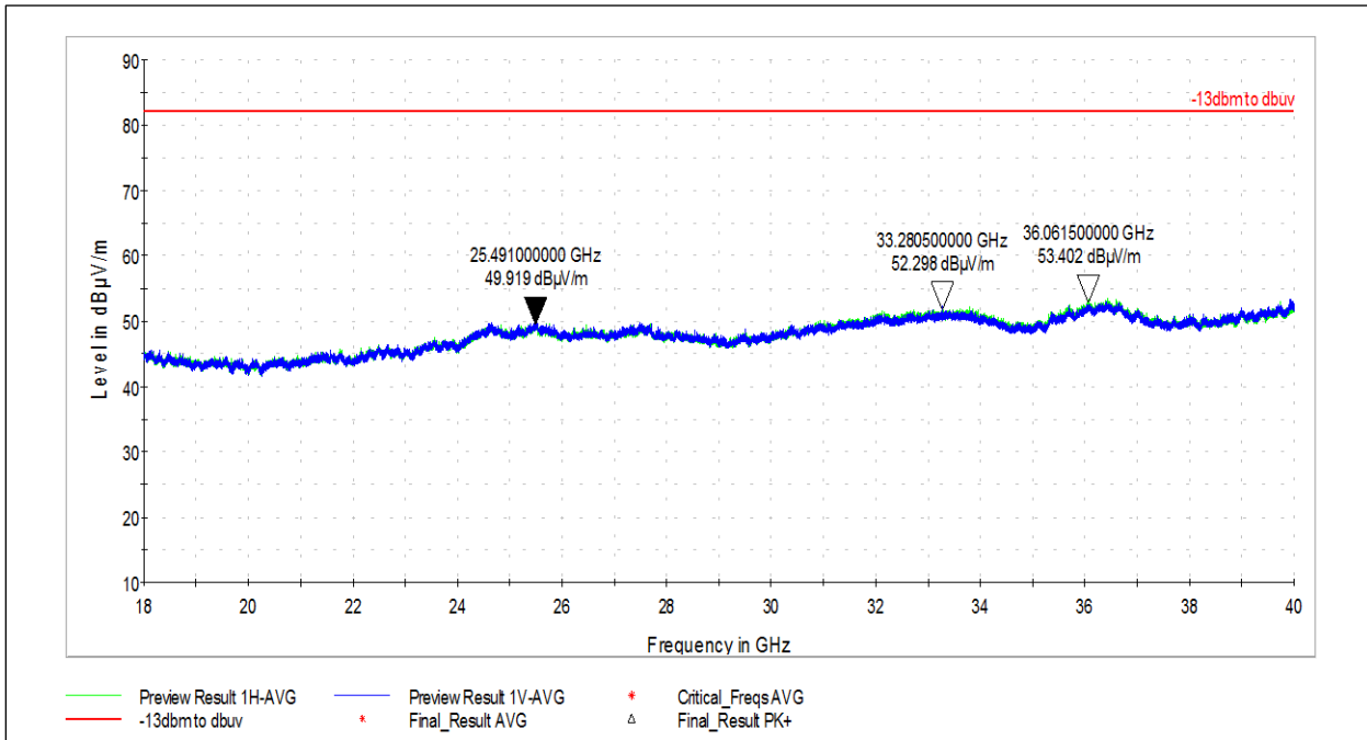
18 – 40GHz Scan (valid for all transmit modes)
