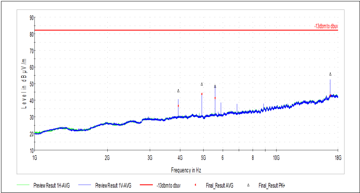
Band n66 Low Channel
