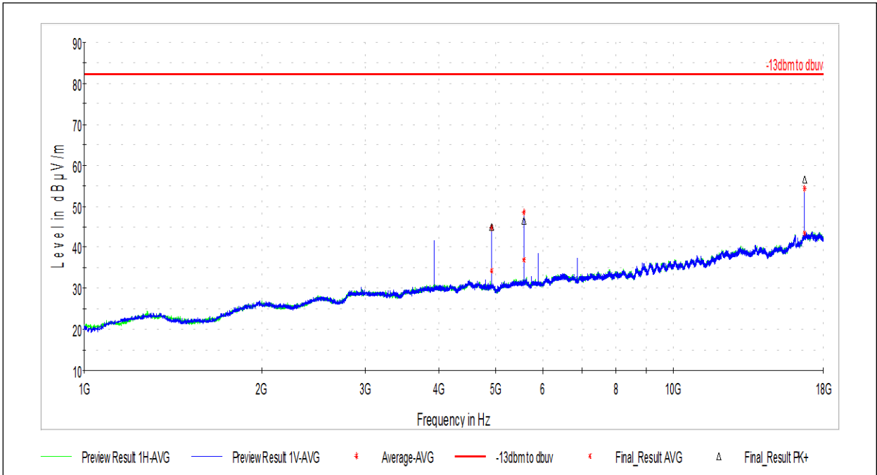
Band n66 Mid Channel
