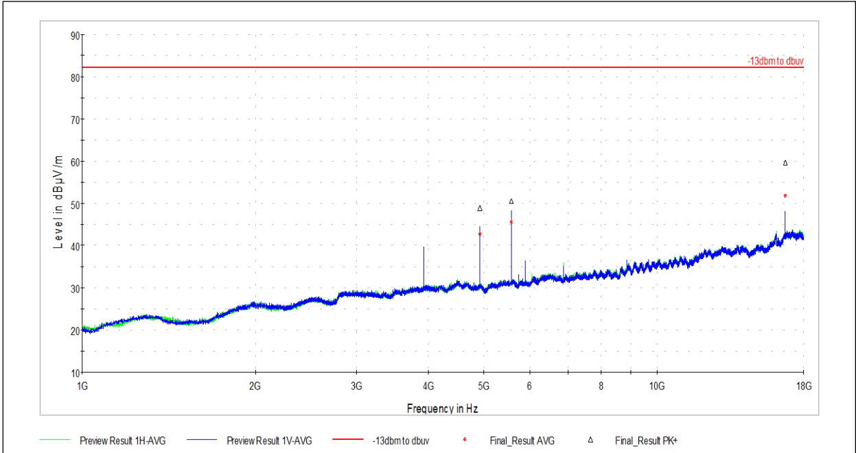
Band n70 High Channel
