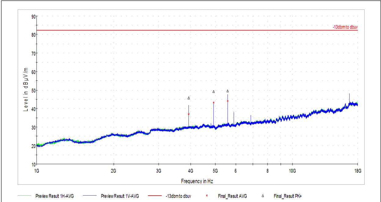
Band n70 Mid Channel
