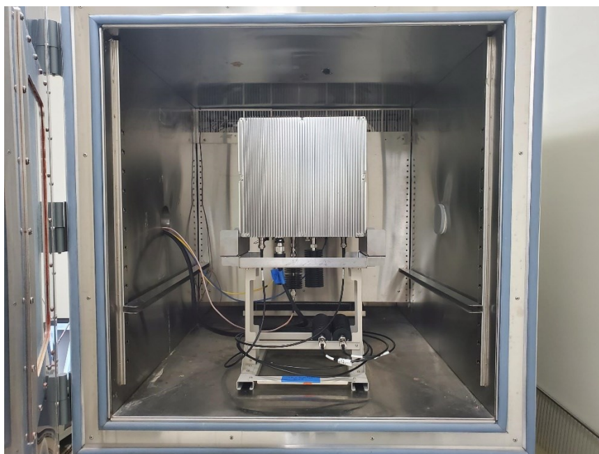
Figure 7 – Test setup – frequency stability measurements
