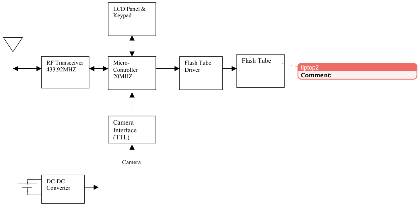
Fig 1. Qflash Trio Circuit Block Diagram
