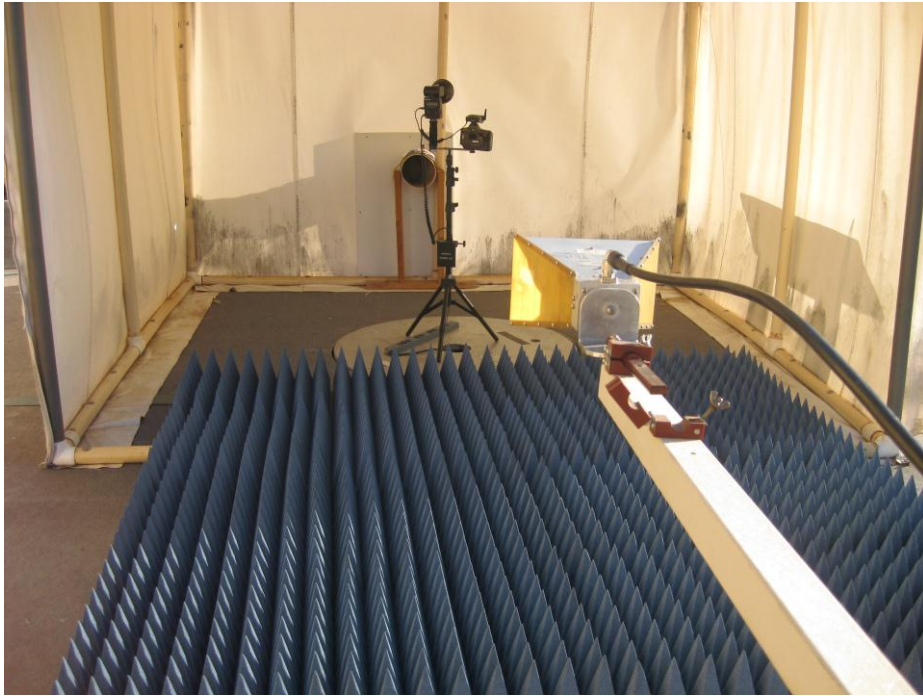
RF Test above 1 GHz
