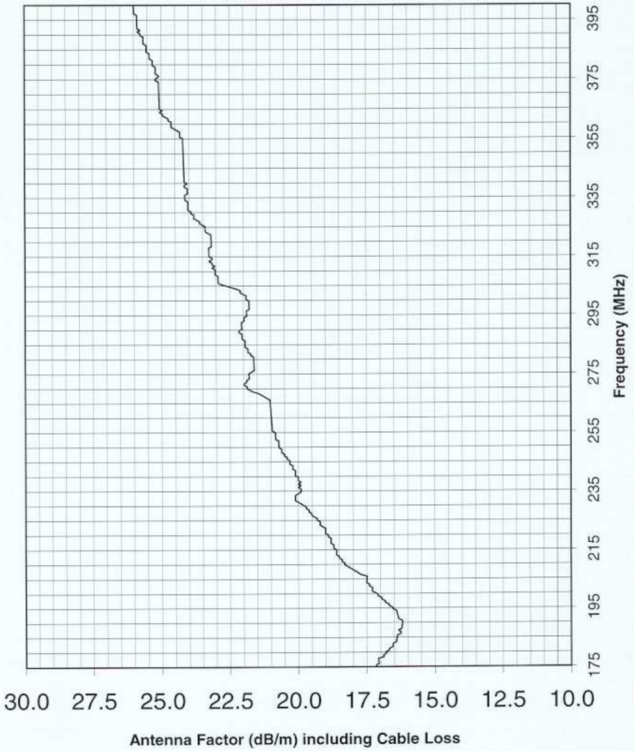
Figure 2.4-4V Compliance Design B200 Antenna Factor Curve Vertical
