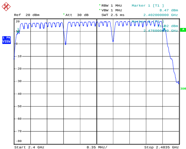
Number of Hopping Channel Plot on Channel 1~36 / 2402 MHz ~ 2476 MHz
