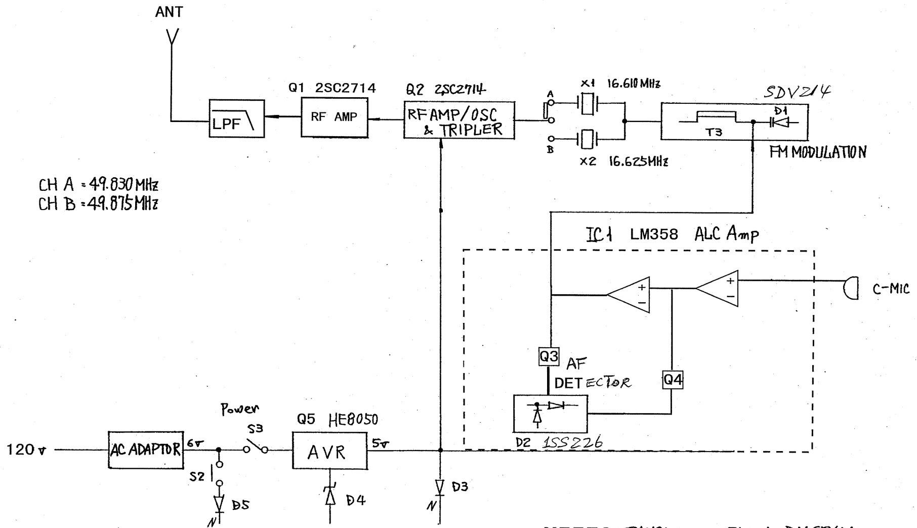
M5578 TRANSMITTER BLOCK DIAGRAM
