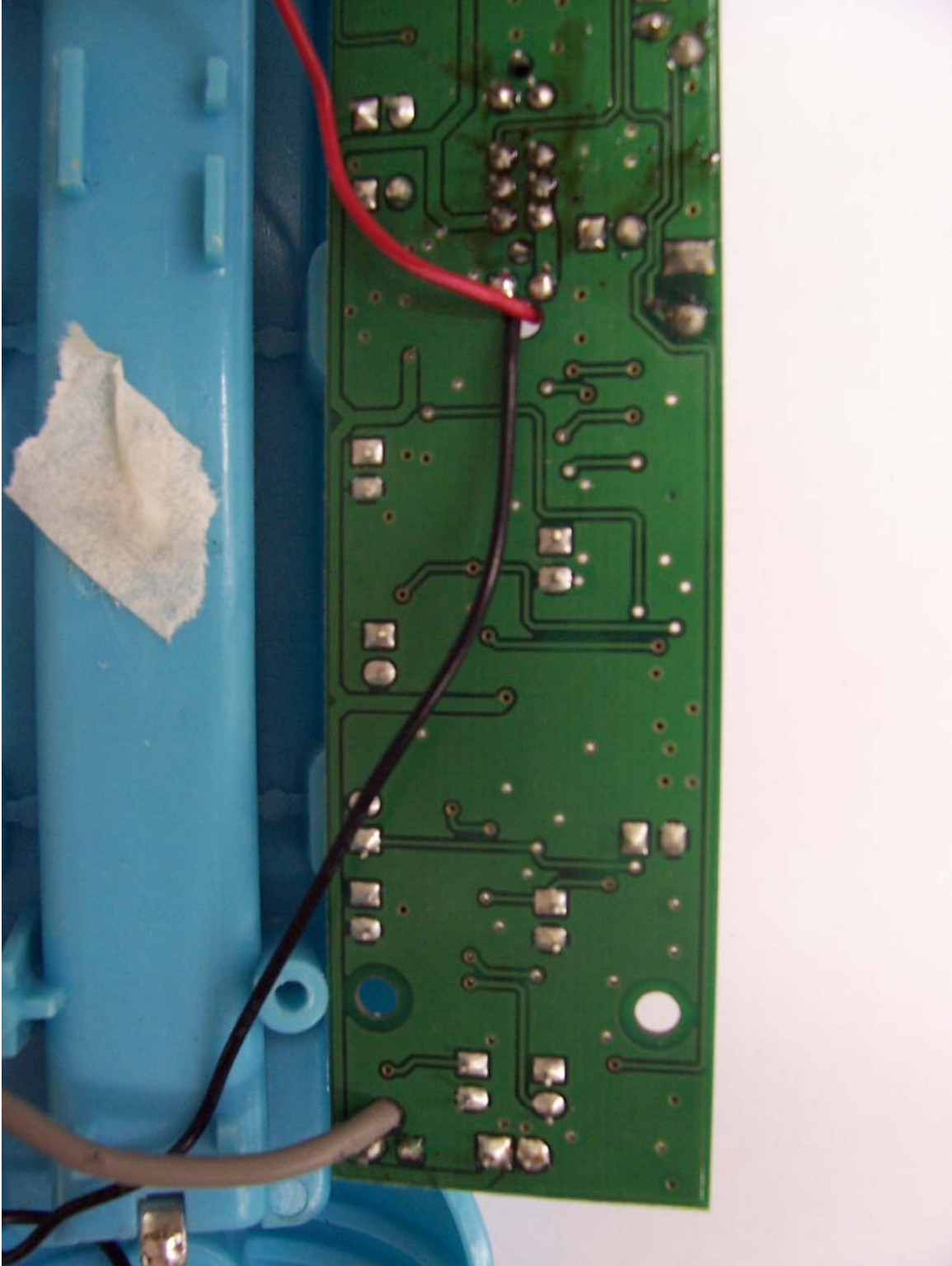
Internal photo Bottom of PCB
