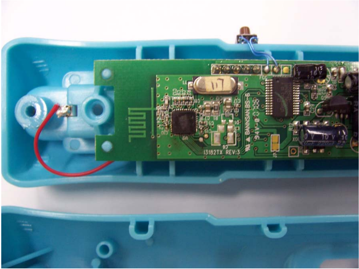
Internal photo Top of PCB Radio Section
