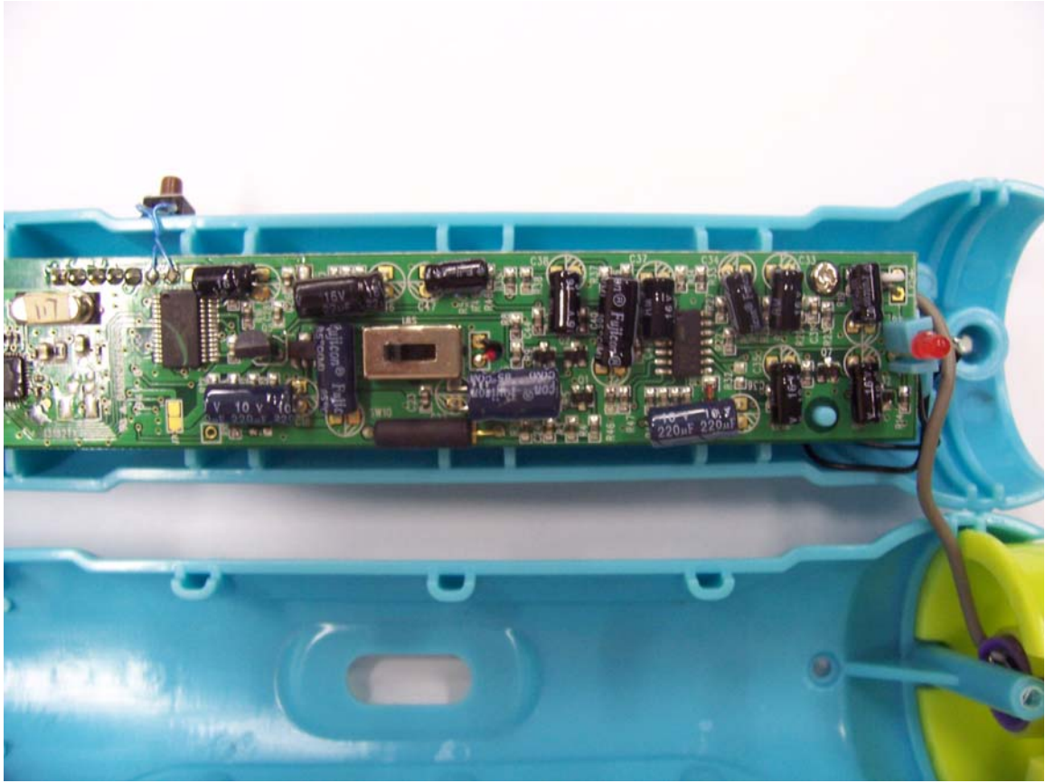
Internal photo Top of PCB
