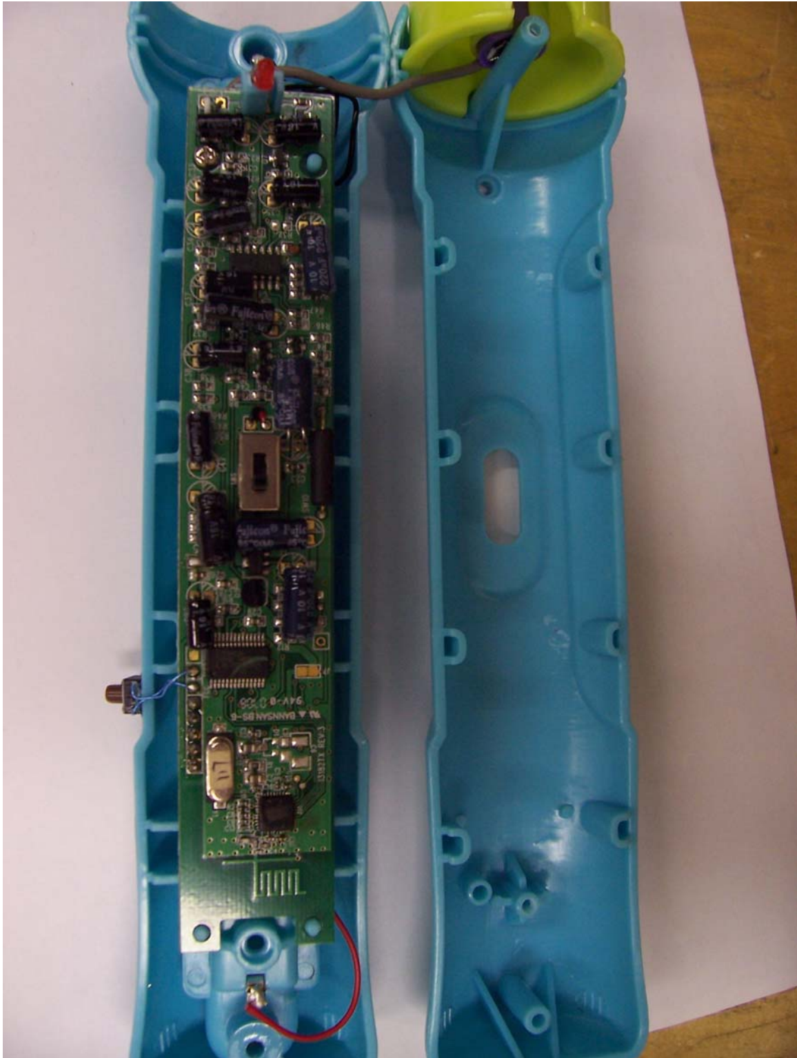
Internal photo Top of PCB
