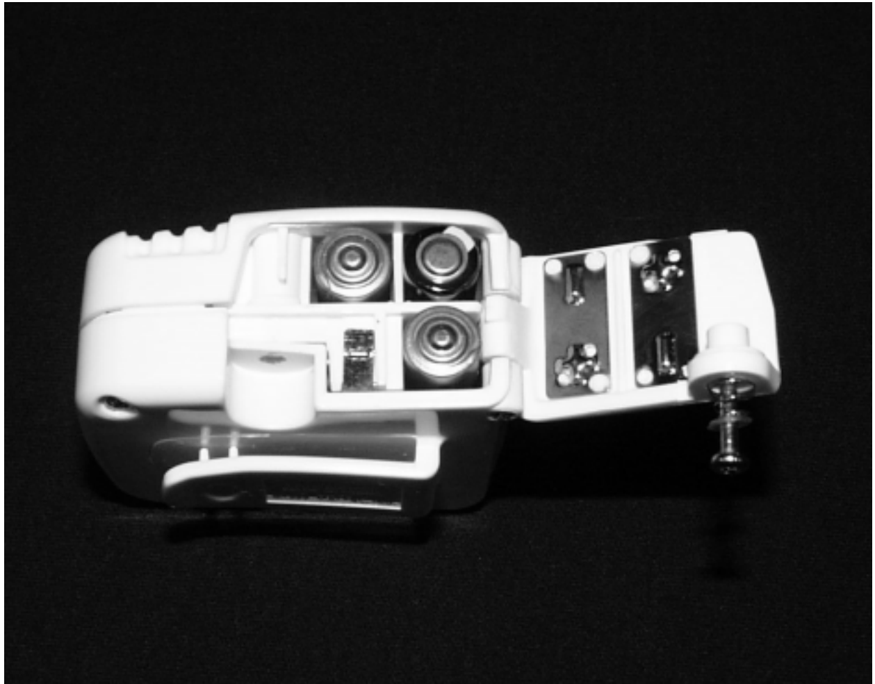
Transmitter, Battery Compartment View
