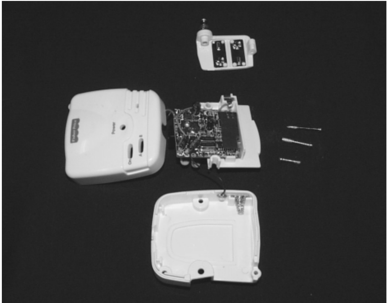
Transmitter, Partially Disassembled
