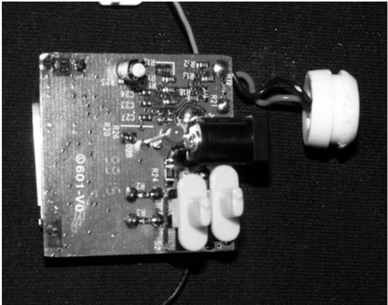
Transmitter, Foil Side of PWB
