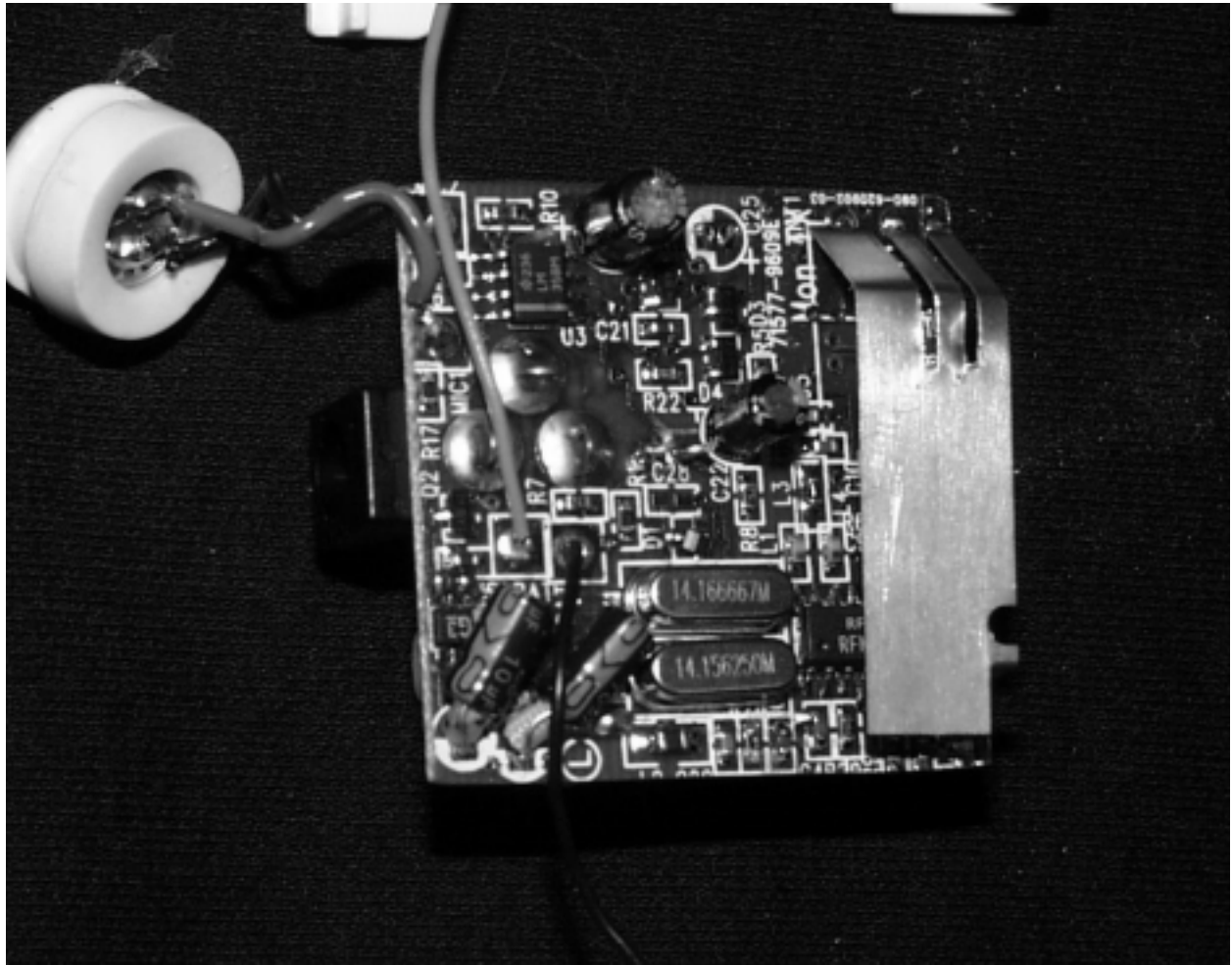
Transmitter, Component Side of PWB
